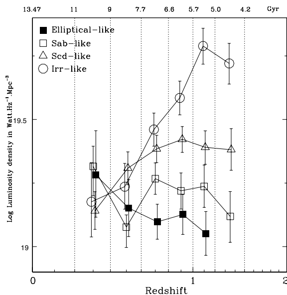
Fig. 7. Comoving non dust-corrected luminosity densities in the rest-frame B -passband from early to late galaxy types (see details in Sect. 6.1). For clarity, data are represented by symbols slightly displaced horizontally from the center of the redshift bins. Error bars are at 1\sigma . The irregular-like type emissivity decreases markedly by a factor 4, while the elliptical-like type increases by a factor 1.7 from z = 1.1 to z = 0.2 . We note that at z < 0.4 the total emissivity is dominated by the early-type population.
