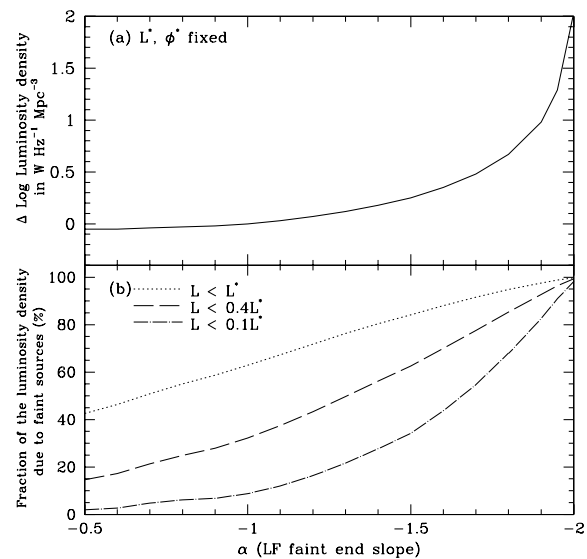
Fig. 1. a). Quantitative change in log of the comoving luminosity density, \mathcal{L} , as a function of the faint-end slope, \alpha , of the LF for fixed L^* and \phi^* values, compared to \log \mathcal{L} for \alpha = -1 . b) Fraction of \mathcal{L} as a function of \alpha due to sources fainter than L^* (dotted line), 0.4L^* (dashed line), and 0.1L^* (dot-dashed line).
