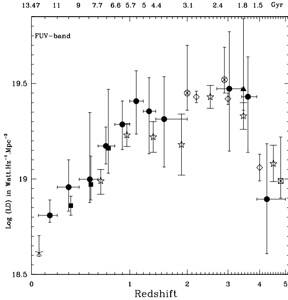
Fig. 9. Comoving non dust-corrected FUV luminosity densities from z = 0 to z = 5 . The plain circles represent the 1500 Å VVDS data ( 0.05 < z < 5 ) (see values and error bars in Tables 1 & 4), the plain triangle represents the 1500 Å VVDS data at 3 < z < 4 derived as in Paltani et al. (2007), and the plain squares represent the 1500 Å GALEX-VVDS data at z < 1 , plotted at +0.02 in redshift for clarity, from Schiminovich et al. (2005). Other data are the 1500 Å GALEX-2dFGRS from Wyder et al. (2005) (asterisk), the 1500 Å HDF data from Arnouts et al. (2005) (crossed circles), the 1700 Å KDF data from Sawicki & Thompson (2006b) (open rhombus), the 1500 Å FDF data from Gabasch et al. (2004) (open stars), and the 1700 Å data from Iwata et al. (2007) (crossed square).
