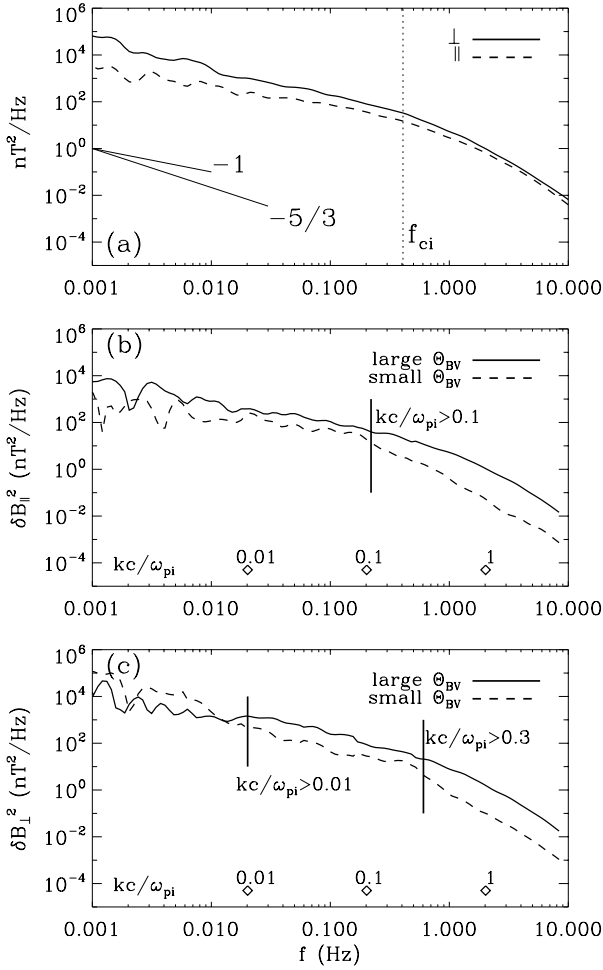
Fig. 5. Same as Fig. 4, but for FGM/Cluster data on 16 December 2001, 05:30–06:30 UT.
