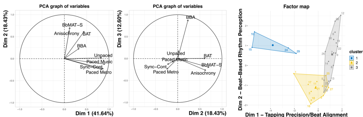
Figure 3. Dimensions (1, 2, and 3) and clusters (1, 2, and 3) for A) the perception PCA and B) the perception + production PCA. A) In the perception PCA, Cluster 1 reflects weak perceivers , Cluster 2 reflects strong sequence memory-based rhythm perceivers , and Cluster 3 reflects strong beat-based rhythm perceivers . B) In the perception + production PCA, Cluster 1 reflects weak tappers , Cluster 2 reflects weak perceivers , and Cluster 3 reflects participants with strong rhythm (perception and production) . Note that only Dimensions 1 and 2 are shown for the cluster graphs for clarity, but Dimension 3 for the perception + production PCA can be seen in Supplementary Figure 3.
