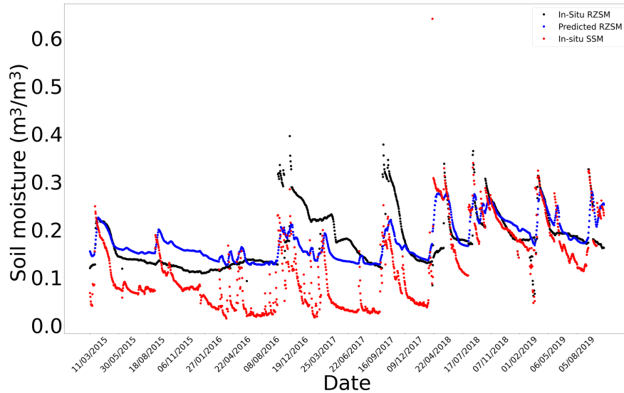
Figure G9. In situ SSM, in situ RZSM, and predicted RZSM series at station P12 (Tunisia) with model ANN_SSM.
