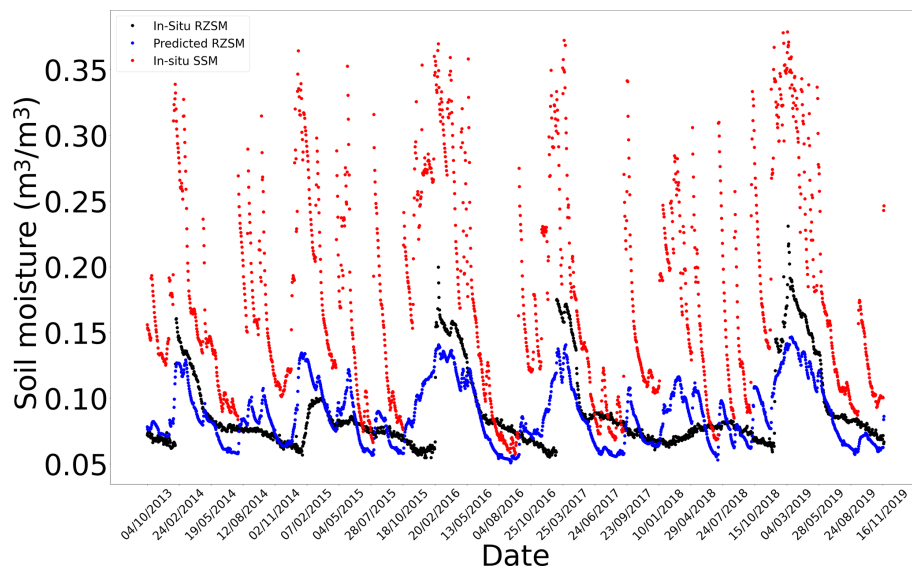
Figure E8. In situ SSM, in situ RZSM, and predicted RZSM series at station Nephi (SCAN) with model ANN_SSM_NDVI_EVAP-EFF-B60_EXP-FILT-T5.
