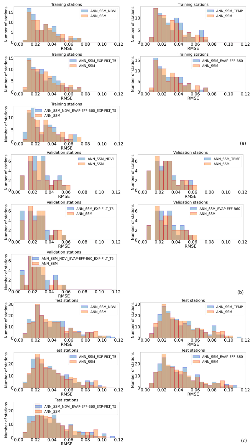
Figure D1. RMSE histograms of all tested ANN models compared to ANN_SSM (a) on training stations, (b) on validation stations and (c) on test stations.
