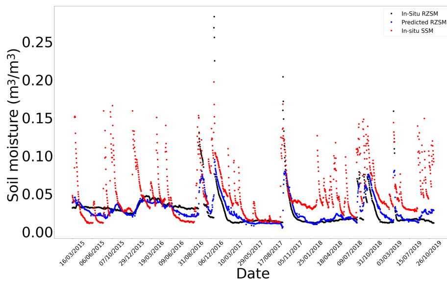
Figure G4. In situ SSM, in situ RZSM, and predicted RZSM series at station Barrouta_160 (Tunisia) with model ANN_SSM_NDVI_EVAP-EFF-B60_EXP-FILT-T5.
