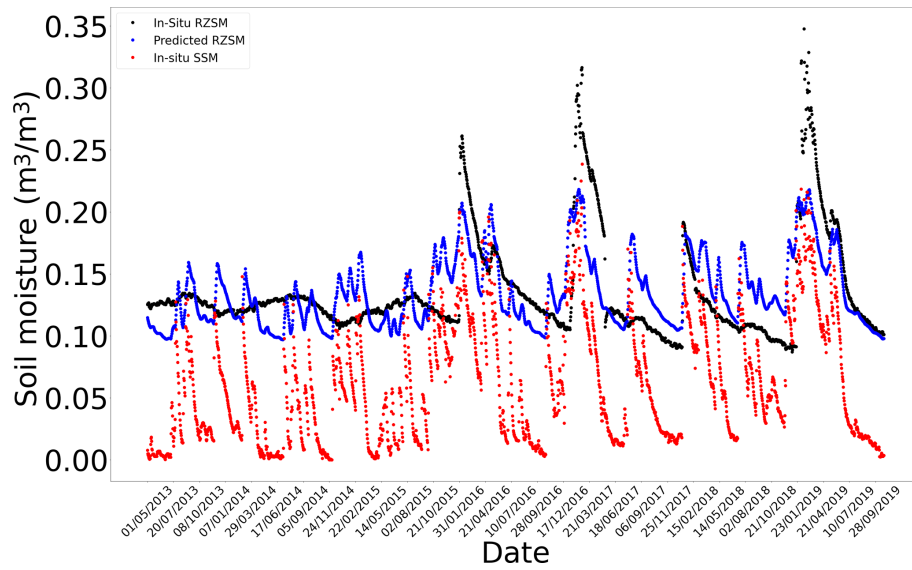
Figure F3. In situ SSM, in situ RZSM, and predicted RZSM series at station PineNut with model ANN_SSM.
