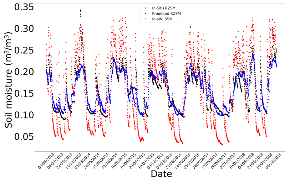
Figure E6. In situ SSM, in situ RZSM, and predicted RZSM series at station Cabrieres D'Avignon (SMOSMANIA) with model ANN_SSM_NDVI_EVAP-EFF-B60_EXP-FILT-T5.
