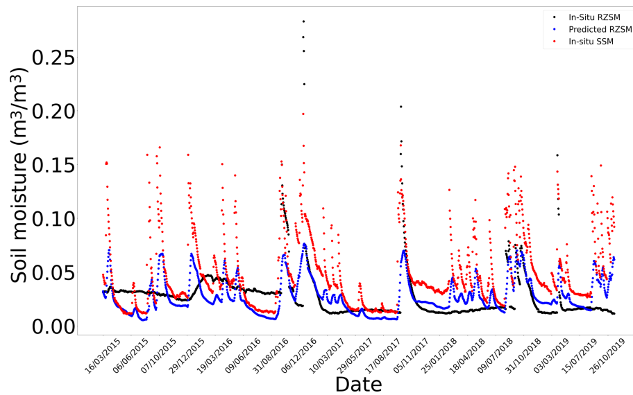
Figure G3. In situ SSM, in situ RZSM, and predicted RZSM series at station Barrouta_160 (Tunisia) with model ANN_SSM.
