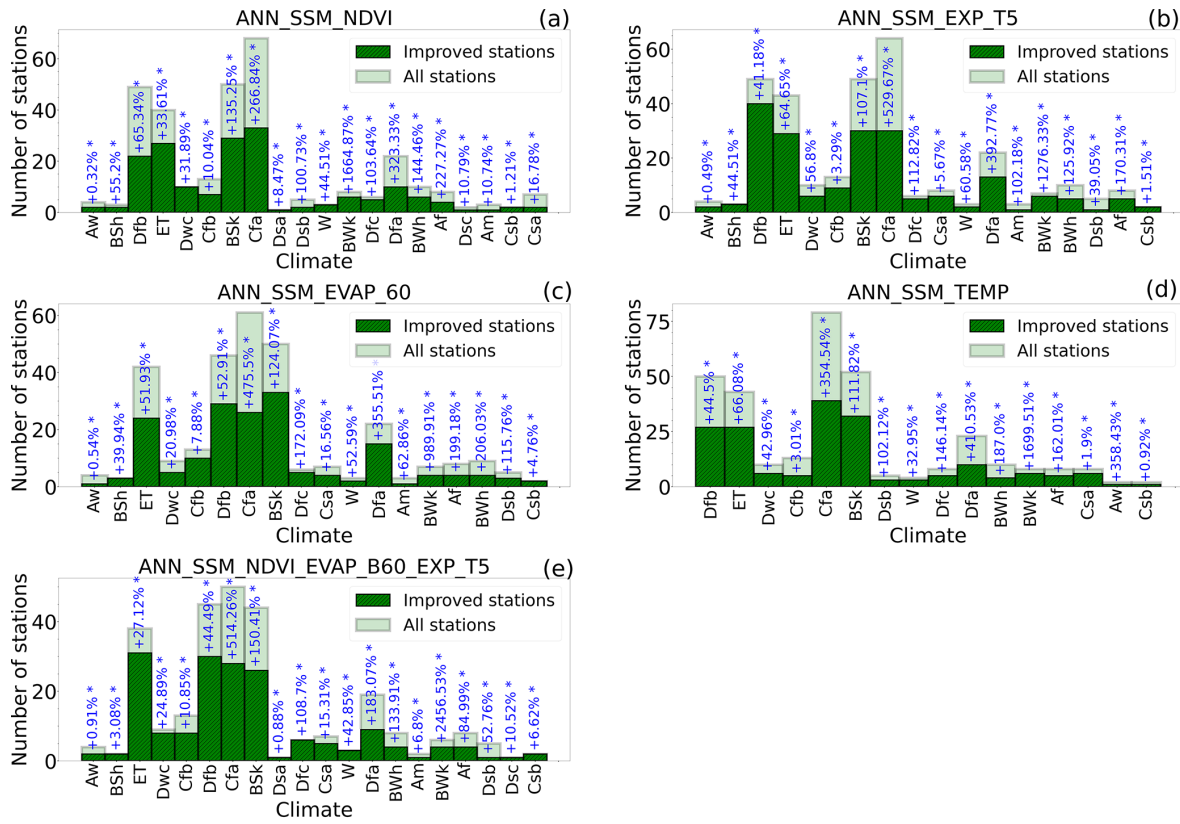
*Mean correlation change rate per climate class
