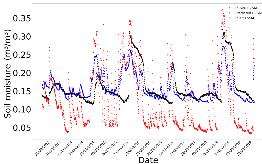
Figure E3. In situ SSM, in situ RZSM, and predicted RZSM series at station HarmsWay (SCAN) with model ANN_SSM.
