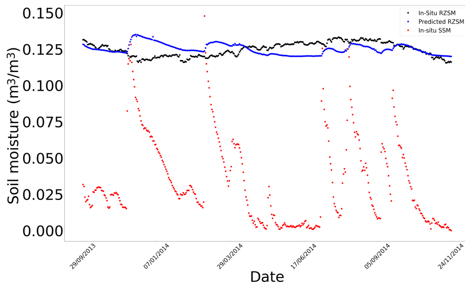
Figure F4. In situ SSM, in situ RZSM, and predicted RZSM time series at the stations in the Kairouan Plain (Tunisia) with model ANN_SSM_NDVI_EVAP-EFF-B60_EXP-FILT-T5 (see Appendix G for a larger figure format).
