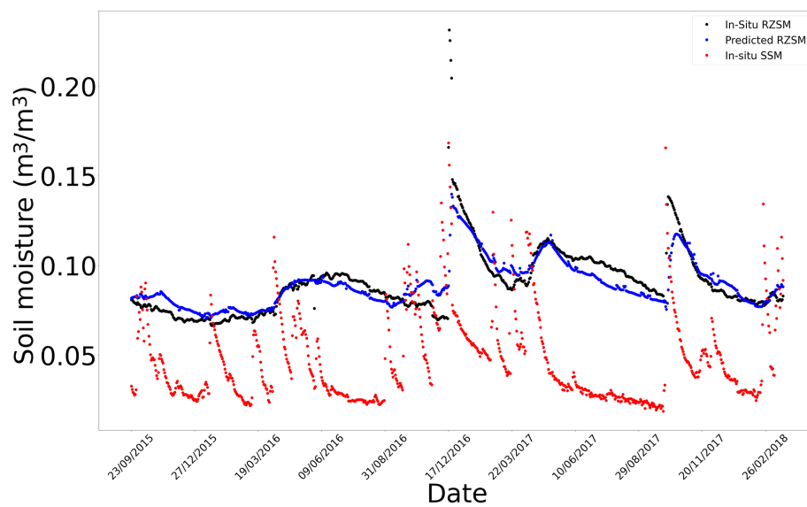
Figure G8. In situ SSM, in situ RZSM, and predicted RZSM series at station Hmidate_163 (Tunisia) with model ANN_SSM_NDVI_EVAP-EFF-B60_EXP-FILT-T5.
