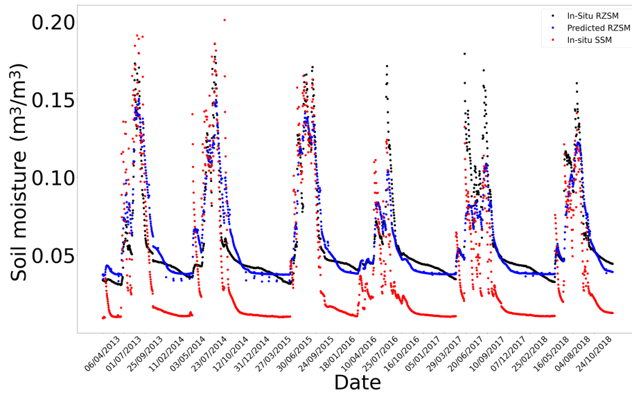
Figure E10. In situ SSM, in situ RZSM, and predicted RZSM series at station Wankama (AMMA-CATCH) with model ANN_SSM_NDVI_EVAP-EFF-B60_EXP-FILT-T5.
