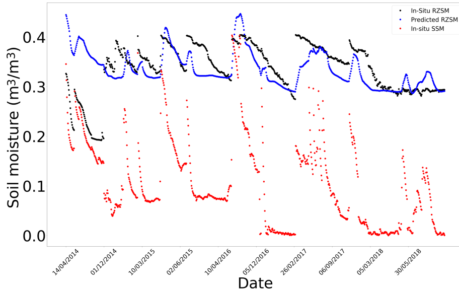
Figure F5. In situ SSM, in situ RZSM, and predicted RZSM series at station S-Coleambally with model ANN_SSM.
