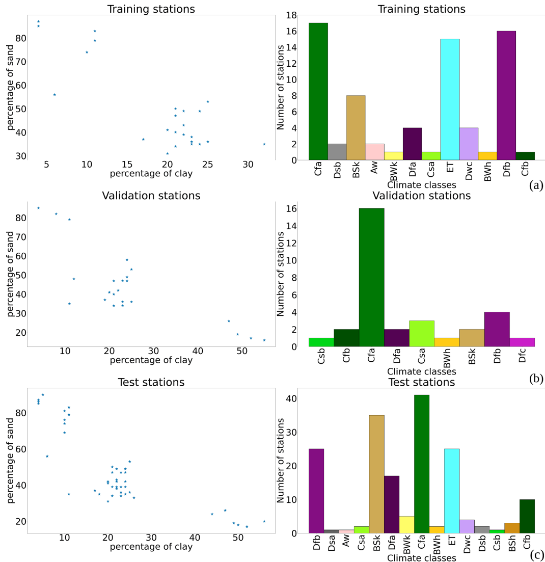
Figure B1. Climate and soil texture for (a) training stations, (b) validation stations and (c) test stations.
