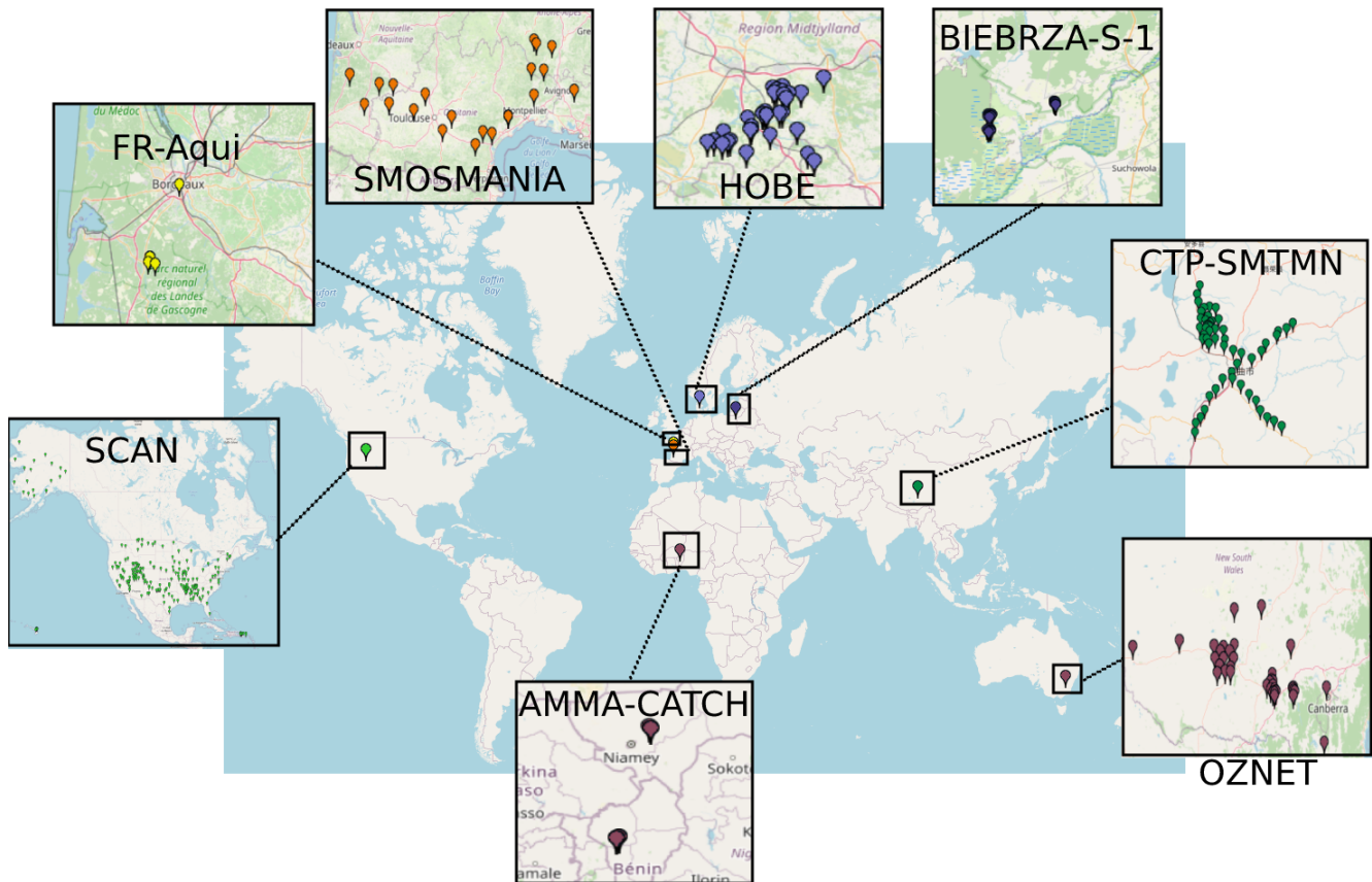
Figure 2. International Soil Moisture Network (ISMN) network distribution (adapted from the ISMN web data portal: https://www.geo.tuwien.ac.at/insitu/data_viewer/ , last access: 7 April 2022; scale: 1 cm = 1000 km).
