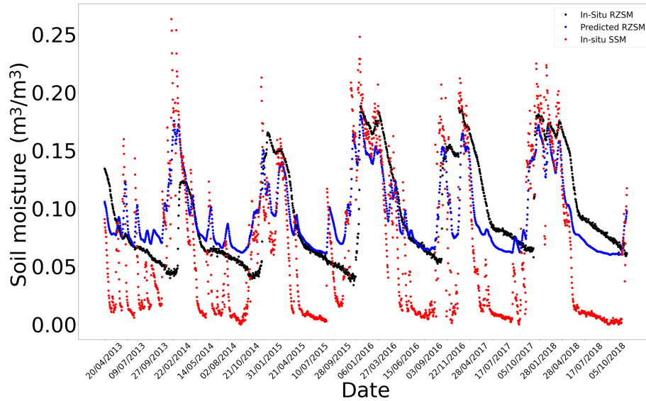
Figure F1. In situ SSM, in situ RZSM, and predicted RZSM series at station Lind#1 with model ANN_SSM.
