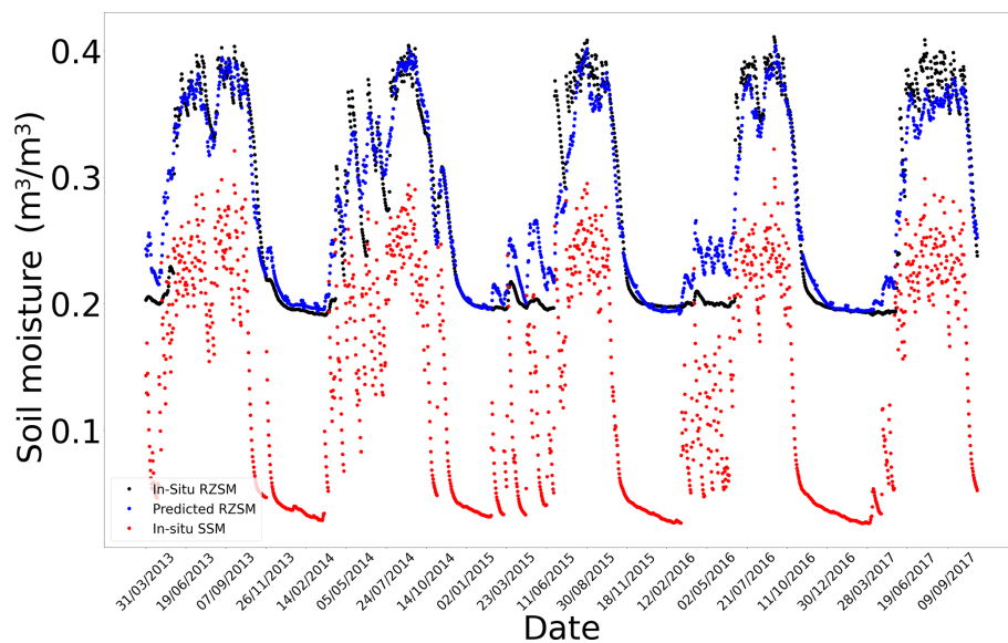
Figure E2. In situ SSM, in situ RZSM, and predicted RZSM series at station Beloufougou Mid (AMMA-CATCH) with model ANN_SSM_NDVI_EVAP-EFF-B60_EXP-FILT-T5.
