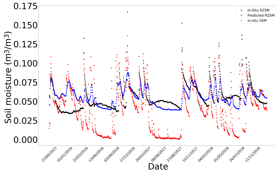
Figure G5. In situ SSM, in situ RZSM, and predicted RZSM series at station Bouhajla_164 (Tunisia) with model ANN_SSM.
