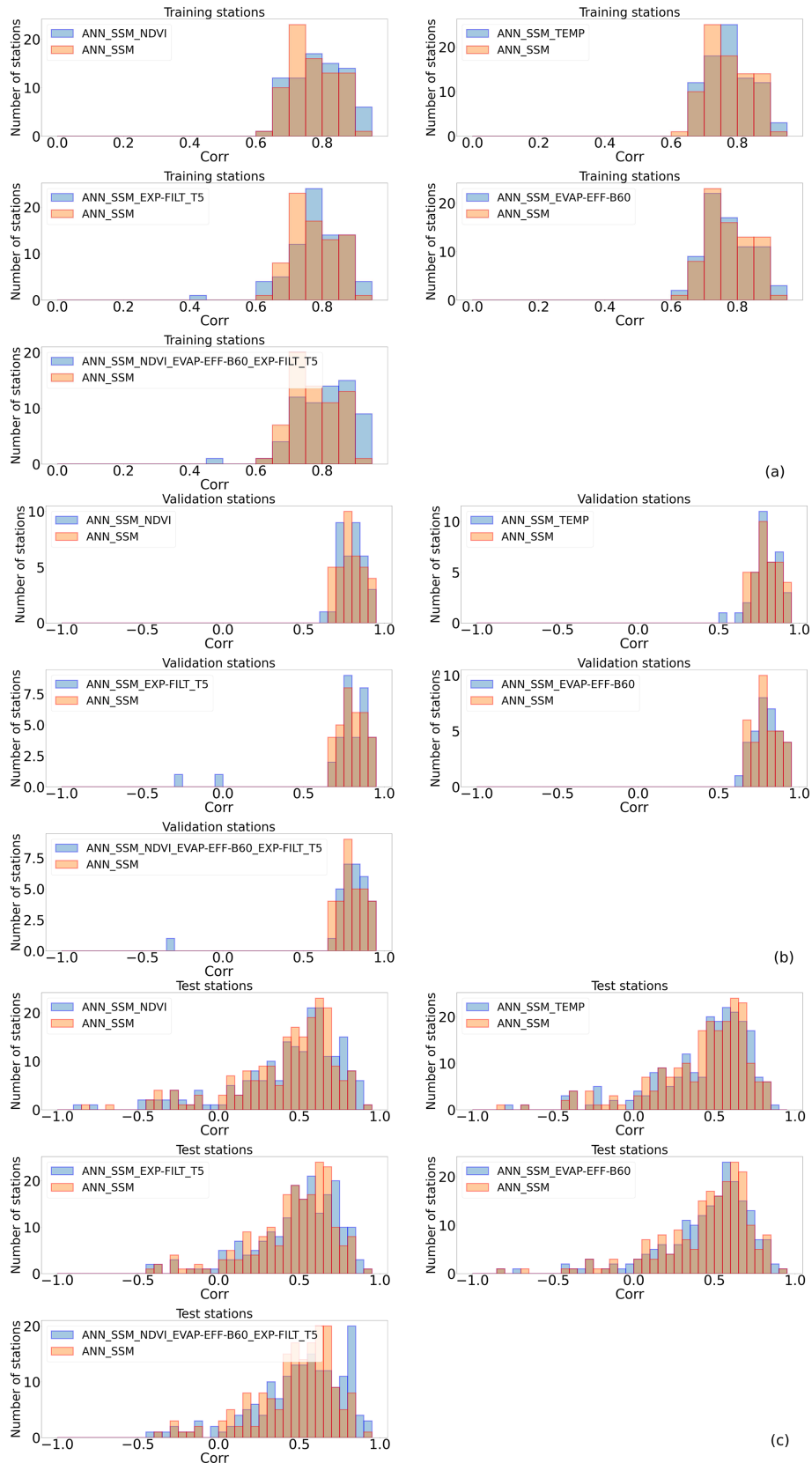
Figure 3. Correlation histograms of all tested ANN models compared to ANN_SSM (a) on training stations (b), on validation stations (c) and on test stations (see Appendix D for RMSE histograms).
