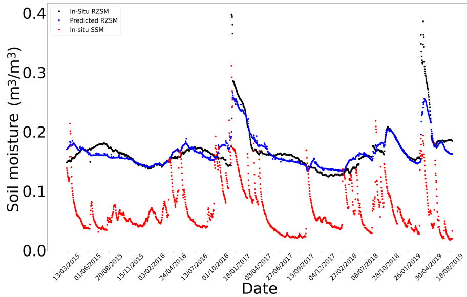
Figure G2. In situ SSM, in situ RZSM, and predicted RZSM series at station Barrage-162 (Tunisia) with model ANN_SSM_NDVI_EVAP-EFF-B60_EXP-FILT-T5.
