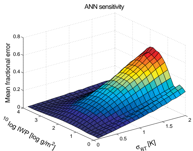
Fig. 11. ANN sensitivity to errors in the input brightness temperatures. Here, only the MHS channels are used as input to the ANN. See the text for an explanation and a discussion.
