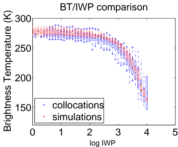
Fig. 8. Modified boxplot of Ice Water Path and MHS channel 5 or AMSU-B channel 20 brightness temperature. Radiances are binned in ^{10}\log IWP bins with a width of 0.1 \log \text{ g/m}^2 . In each bin, the median brightness temperature is shown as a horizontal line. The upper and lower bars of the rectangle show the 1st and 3rd quartile (25th and 75th percentile). From the rectangles, dashed lines connect to the 1st and 99th percentile. All other points are defined as outliers and plotted as pluses. Collocations are shown in blue and simulations are shown in red.
