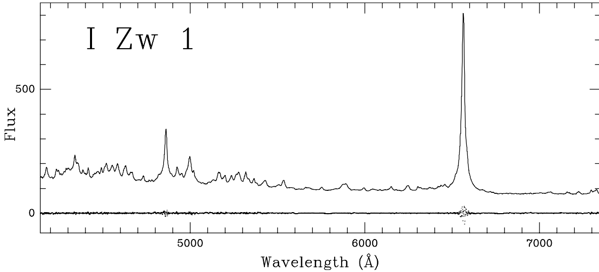
Fig. 1. The deredshifted AAT spectrum of I Zw 1 with the residuals. The fit is not shown. The fluxes are in units of 10^{-16} erg \text{cm}^{-2} \text{Å}^{-1} \text{s}^{-1} .
