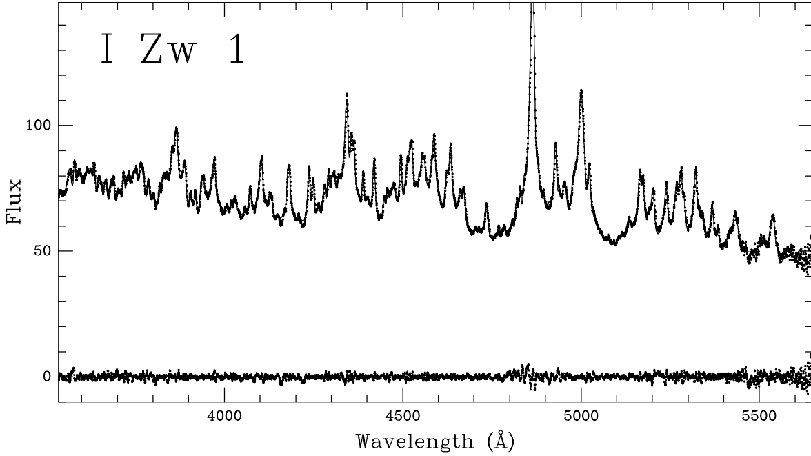
Fig. 3. The deredshifted blue WHT spectrum of I Zw 1 (dots), the best fit and the residuals. The fluxes are in units of 10^{-16} \text{ erg cm}^{-2} \text{ \AA}^{-1} \text{ s}^{-1} .
