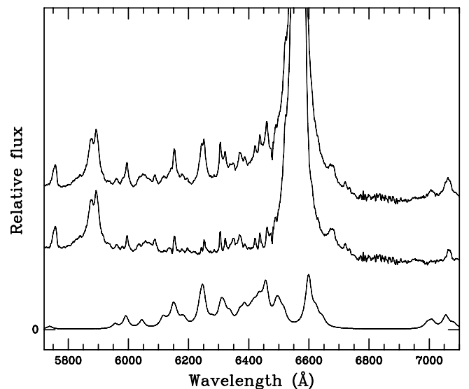
Fig. 7. This figure shows the red deredshifted WHT spectrum of IZw 1 (top), the synthetic broad line Fe II spectrum, uncorrected for reddening (bottom) and the difference (middle), shifted downward for clarity.
