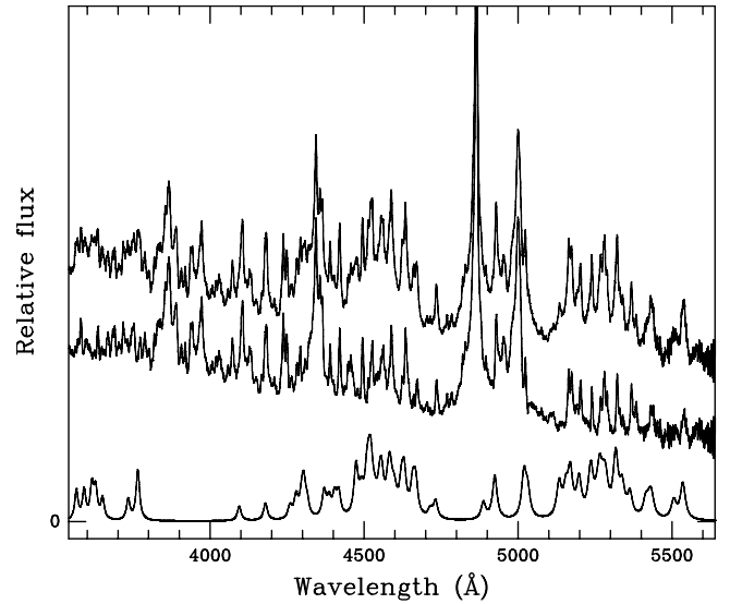
Fig. 6. This figure shows the blue deredshifted WHT spectrum of IZw 1 (top), the synthetic broad line Fe II spectrum built as explained in the text, uncorrected for reddening (bottom) and the difference (middle), shifted downward for clarity.
