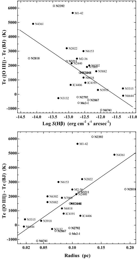
Figure 6. The difference between the nebular electron temperatures derived from the [O III] nebular to auroral forbidden-line ratio, T_e([O III]) , and from the nebular Balmer continuum discontinuity, T_e(BJ) , is plotted against the intrinsic nebular H\beta surface brightness (top) and absolute radius (bottom). Open circles data are from LD93b. The solid lines are the linear fits discussed in the text.
