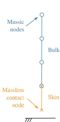
Figure 1: Redistributed mass on a discrete bar
