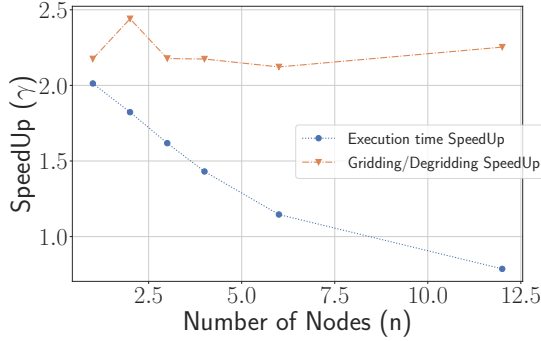
Fig. 9. Speedup of gridding/degriidding and total execution time between 4 MPI processes and 1 MPI process regarding the number of nodes.
