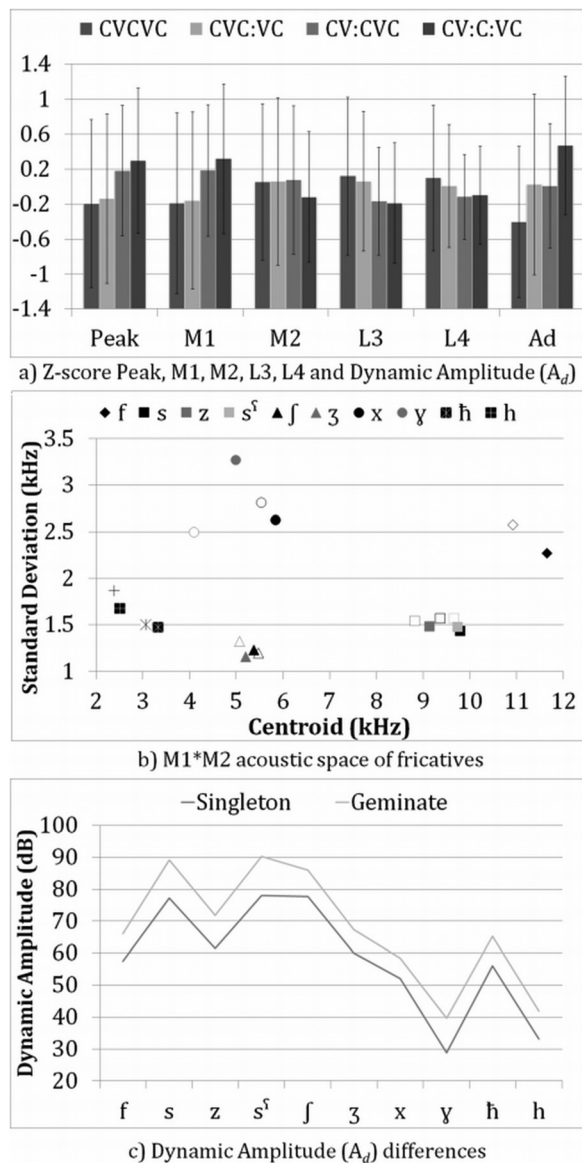
FIG. 5. Z-score of the peak, the four spectral moments and dynamic amplitude ( A_d ) of fricative consonants (a), the (M1*M2) acoustic space of fricative consonants, with geminates in black/gray filled symbols (b), and results of dynamic amplitude ( A_d ) by fricative phonemes in singleton and geminate environments (c).
