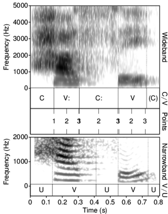
FIG. 1. Wideband spectrogram of the word /ha:tsɛ/ “I feel” produced by a female speaker, and segmentation into C and V (consonant and vowel, respectively, see tier C/V), points of measurements (tier points), followed by a narrowband spectrogram and boundaries for the voiced and unvoiced frames (V and U, respectively, see tier V/U).
