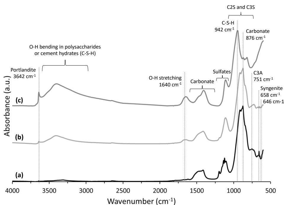
Figure 8. Infrared spectra of (a) anhydrous cement, (b) the matrix with W/C=0.5 and (c) the ITZ.
