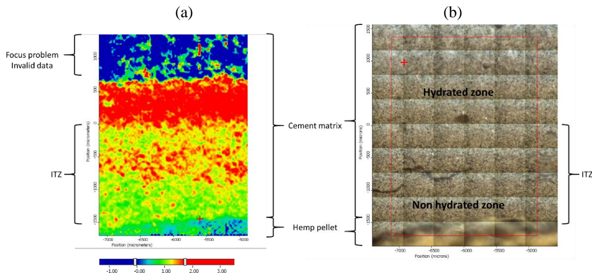
Figure 9. (a) Infrared mapping and (b) zone observed of the vibration band area relative to Portlandite ( 3640\text{ cm}^{-1} ) of a W/C=0.5 sample.
