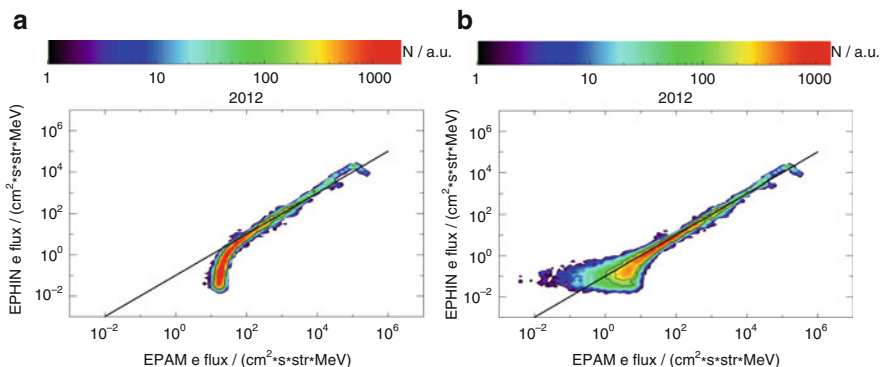
Fig. 7.5 The left panel (a) displays 5 min electron intensities of EPAM (x-axis) and EPHIN (y-axis) plotted against each other. The right panel (b) shows the same plot for background subtracted data
