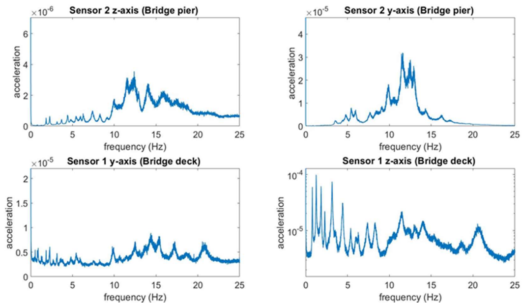
Figure 10: FFT applied to the 4 recorded time series.
