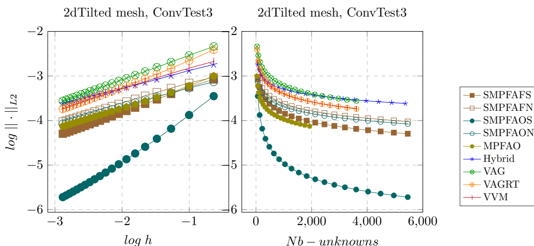
Figure 12: Convergence curves for ConvTest3
