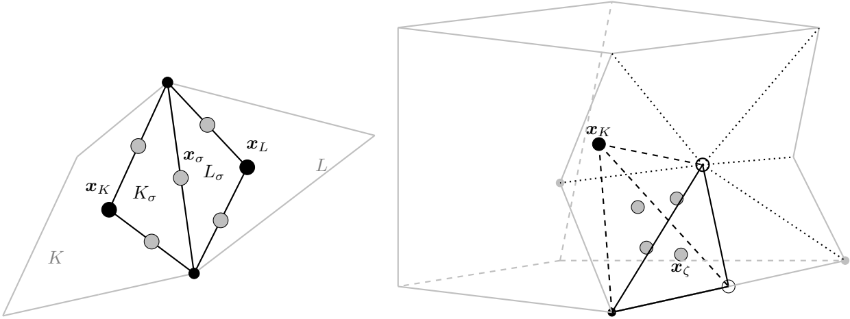
Figure 2: Example of domain D_\sigma in dimension 2 (left) and half domain D_\zeta in dimension 3 (right): empty circles are face centers, grey circles are the location of the unknowns of the local variational problem
