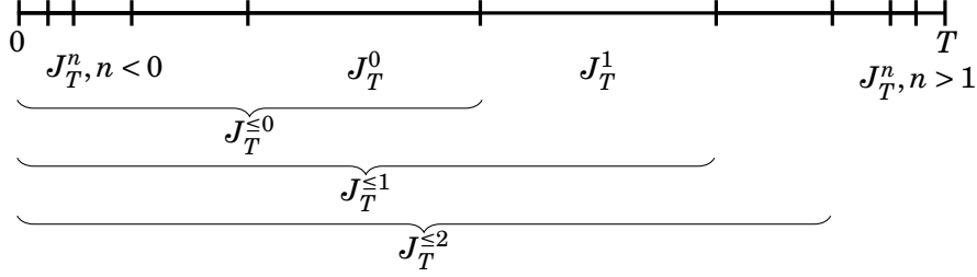
Figure 4: The time intervals J_T^n , n \in \mathbb{Z} .
