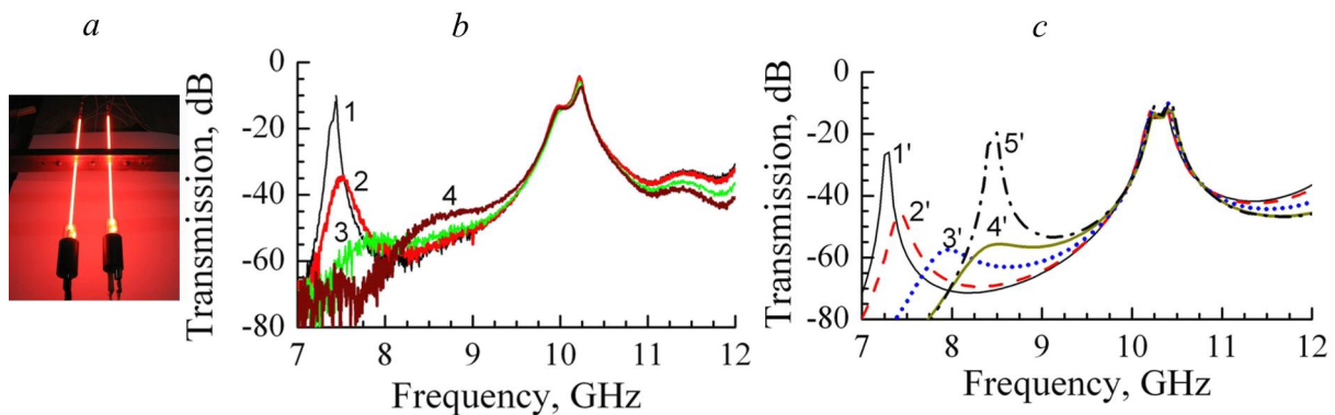
Fig. 4. Photo of waveguide section with 2 lamps and 3 rods ( a ) and corresponding experimental ( b ) and calculated ( c ) transmittance spectra.
