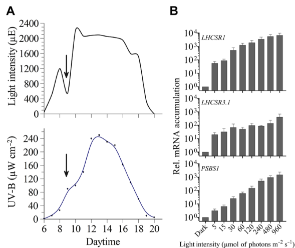
Fig. 1. PAR and UV-B intensity from sunrise to sunset and changes in LHCSR and PSBS1 transcript levels after irradiation at various light intensities.
