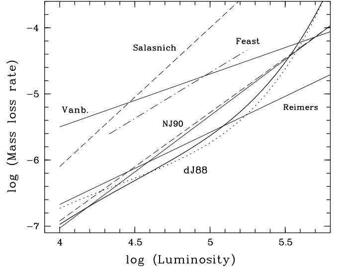
Fig. 1. Comparison of several prescriptions for the RSG mass-loss rates (unit M_{\odot} \text{ yr}^{-1} ) plotted against luminosity (in L_{\odot} ). The de Jager prescription is represented by the two curved lines (solid line T_{\text{eff}} = 4000 \text{ K} , dotted line T_{\text{eff}} = 3500 \text{ K} ).
