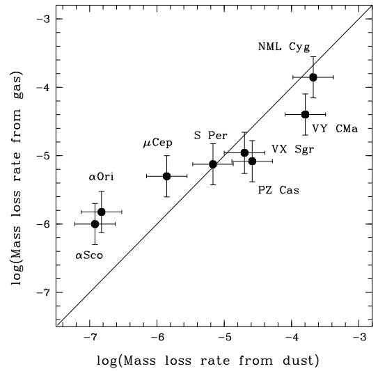
Fig. 4. Mass-loss rates from observation of the gas versus mass-loss rate from observation of the dust (the 60 \mu\text{m} emission) for the eight RSGs of Table 2.
