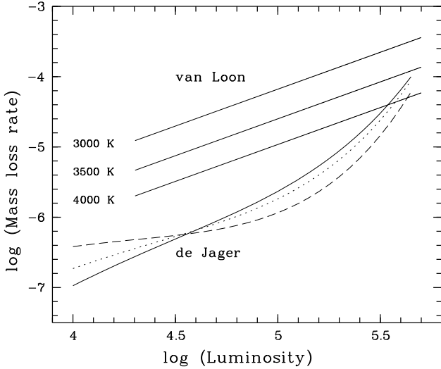
Fig. 6. Mass-loss rate prescription of van Loon et al. (2005) and de Jager (1988) with \dot{M} plotted as a function of luminosity and for three values of T_{\text{eff}} . The de Jager lines are solid, dotted and dashed for 4000, 3500 and 3000 K respectively.
