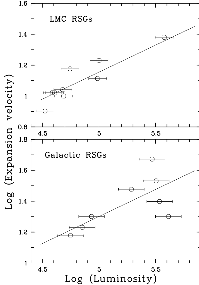
Fig. C.1. Wind expansion velocity, in \text{km s}^{-1} , as a function of luminosity (in L_{\odot} ), for Galactic RSGs ( lower panel ), and LMC RSGs ( upper panel ). The straight line for Galactic RSGs corresponds to V = 20 (L/10^5)^{0.35} in \text{km s}^{-1} . The straight line for LMC RSGs corresponds to V = 14 (L/10^5)^{0.35} .
