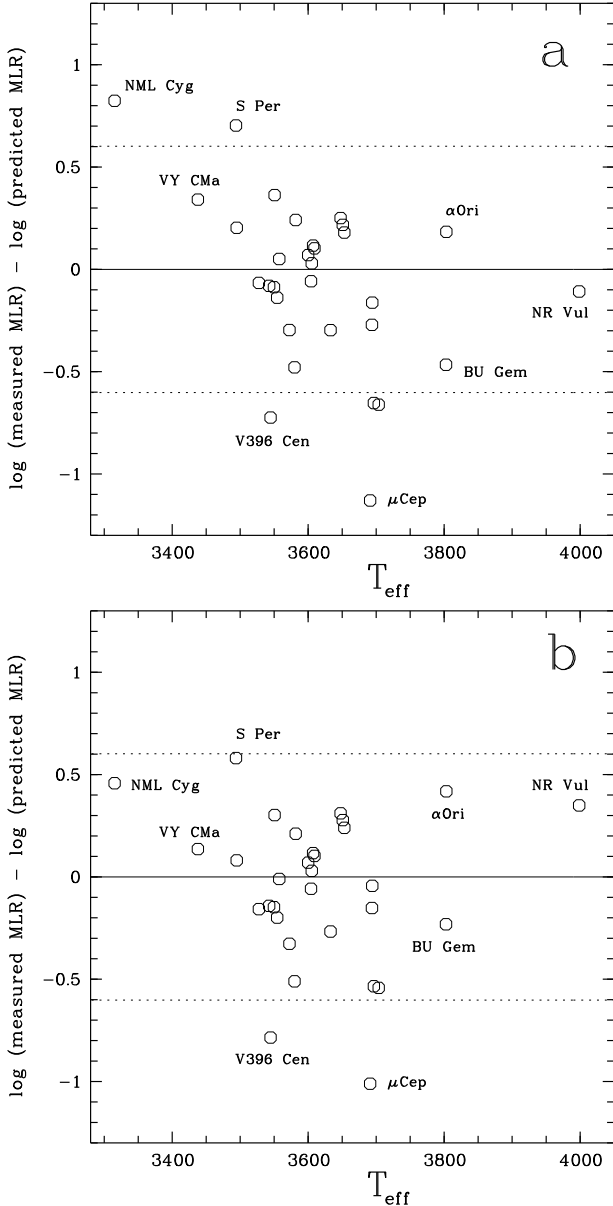
Fig. 7. Panel a ): discrepancies between measured mass-loss rates (MLR) and mass-loss rates predicted by the de Jager prescription, plotted versus T_{\text{eff}} , for Galactic red supergiants. The horizontal dotted lines indicate discrepancies by factors 4 and 1/4. Panel b ): same as panel a ) when the de Jager rate is multiplied by (T_{\text{eff}}/3600)^{-10} .
