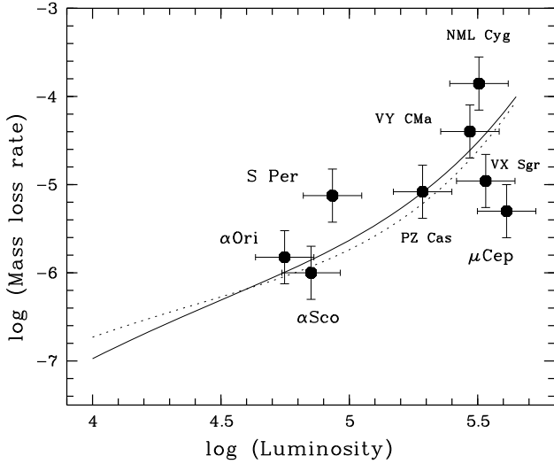
Fig. 3. Mass-loss rates (from observations of the gas) versus luminosity for the eight RSGs of Table 2. The lines are the de Jager rates for 4000 K (solid line) and 3500 K (dotted line).
