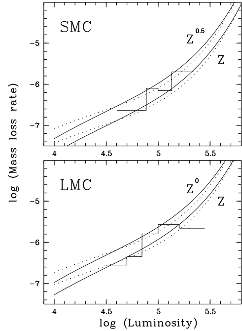
Fig. 8. Mass-loss rates versus luminosity for Magellanic Clouds. The (median) data of Bonanos et al. (2010) are represented by histograms (see text). The solid and dotted lines show the de Jager rates for 3500 and 4000 K scaled for various metallicity dependences, as indicated in the panels.
