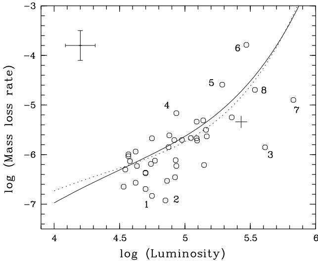
Fig. 2. Comparison of de Jager rate (plotted for T_{\text{eff}} = 3500 K and 4000 K) with mass-loss rates of 39 RSGs listed in Table 1. The mass-loss rates are based on the study of dust and obtained with Jura’s formula. The labels indicate a few wellknown RSGs as follows: 1: \alpha Ori; 2: \alpha Sco, 3: \mu Cep, 4: S Per, 5: PZ Cas, 6: VY CMa, 7: EV Car (at 4.2 kpc); 8: VX Sgr. The small cross represents EV Car if a smaller distance of 2.5 kpc is adopted. At the upper left corner, error bars represent uncertainties of \pm 30 percent in luminosity, and a factor of \pm 2 in \dot{M} .
