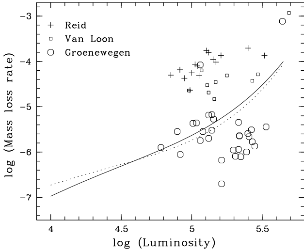
Fig. 5. Mass-loss rates plotted as a function of luminosity for the LMC RSGs. Three samples are plotted: Reid et al. (1990) (15 small crosses), van Loon et al. (2005) (10 small squares), and Groenewegen et al. (2009) (30 circles). The de Jager rates are represented as in previous figures by solid and dotted lines for 4000 K and 3500 K, respectively.
