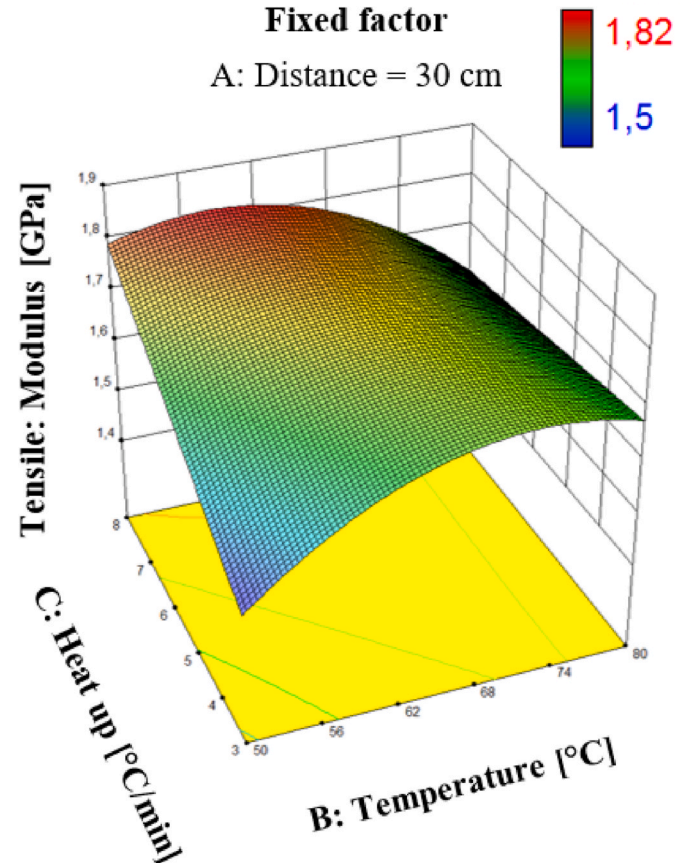
Fig. 9. Influence of the parameters on the measurement of the tensile modulus according to parameter BC.
