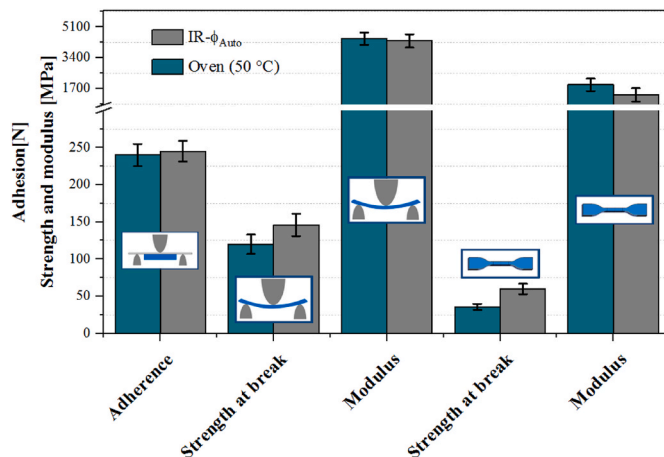
Fig. 6. Some mechanical characteristics of the DGEBA-TETA mixture according to both methods of curing (IR- \Phi_{\text{Auto}} and thermal curing).
