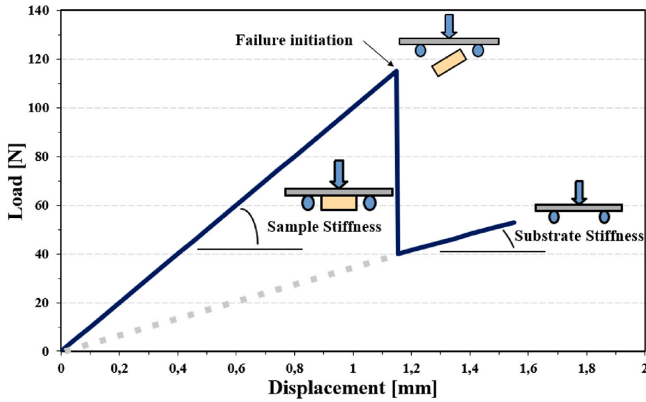
Fig. 2. Illustration of the load-displacement curve for a three-point bending adherence test, highlighting the stiffness of the sample and substrate according to [21].
