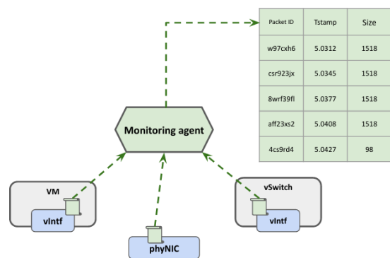
(b) The monitoring agent retrieves the log files from the eBPF programs plugged into the interfaces of the network's nodes, and compiles the parsed information into structured tables.
