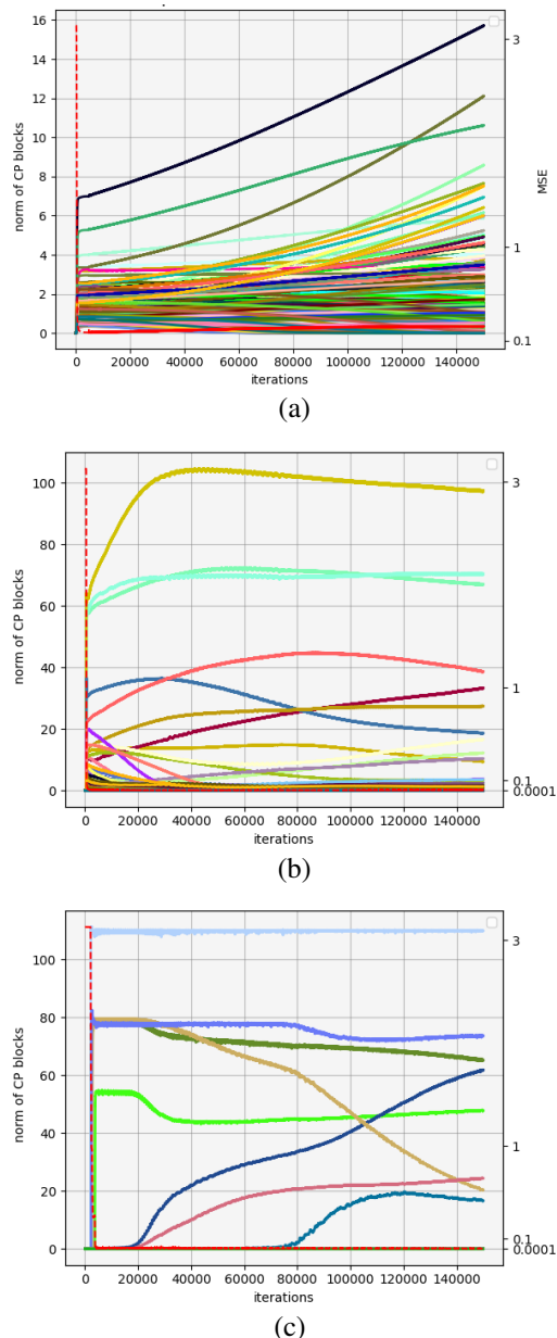
Figure 2. This series of figures compares the learning behaviour for shallow to deep tensors through the evolution of the norms of the blocks along training epochs for depth 0 (a), 1 (b), and 2 (c) for a particular initialization ( \sigma_w = 0.01 , \sigma_A = 0.01 ). Each figure shows 500 curves corresponding to the norm of blocks (y-scale on the left of the plot), plus an additional curve (dotted red line) which stands for the loss (with y-scale on the right of the plot in log-scale).
