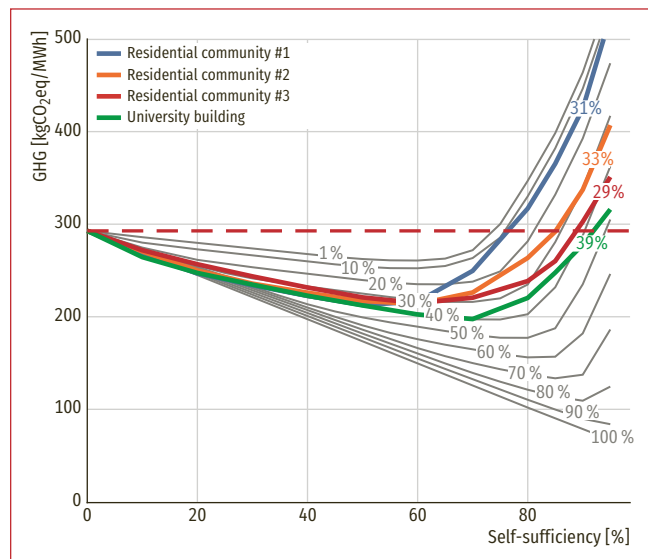
Fig. 3: Verifying the hypothesis on NSS for the German case using four different load profiles with various natural self-sufficiency (specified on each curve). Source: authors' own compilation
