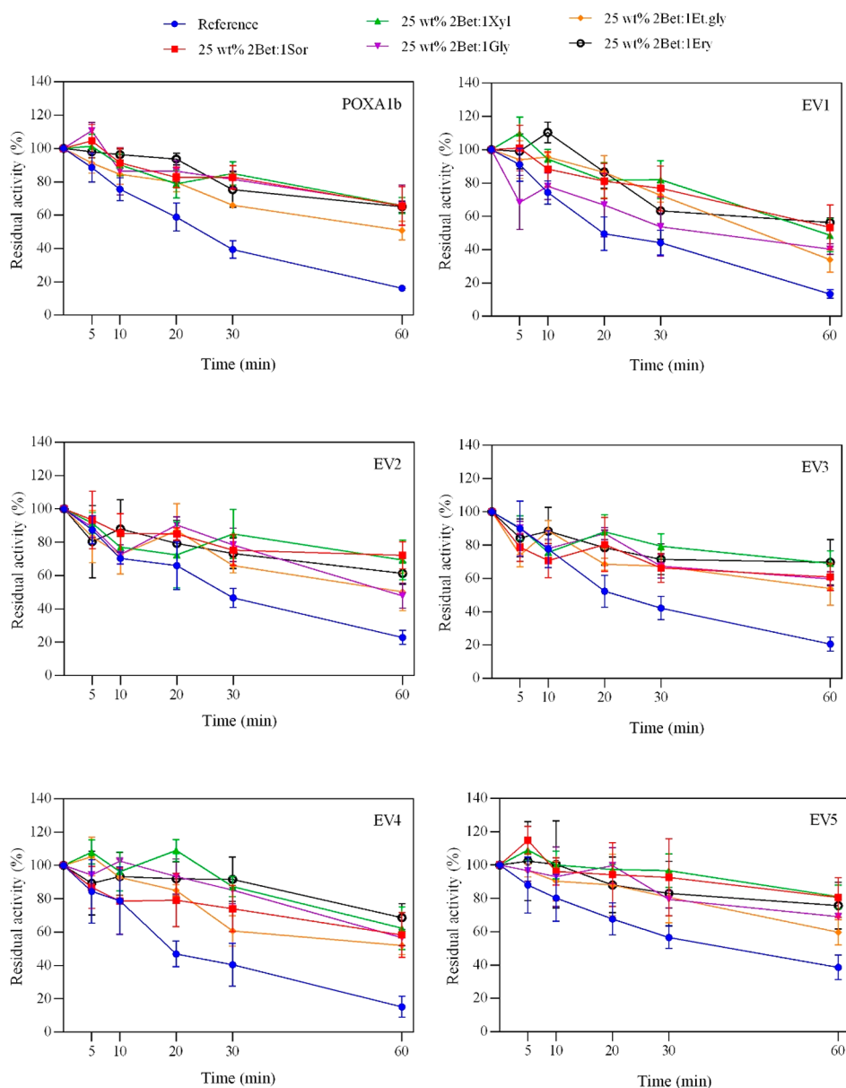
Figure 1. Comparison of thermostability of 1.25 \text{ g L}^{-1} laccases in 50 \text{ mM} phosphate buffer, pH 7 aqueous solution in the absence (blue dots), and in the presence of 25 wt % of 2Bet:1Sor (red squares), 2Bet:1Xyl (green triangles), 2Bet:1Gly (purple triangles), 2Bet:1Et.gly (orange dots), and 2Bet:1Ery (black circles) at 70 \text{ }^\circ\text{C} . The residual activity (%) is determined by comparing the activity measured after a set amount of time with the free-NADES phosphate buffer, pH 7.0 and 50 \text{ mM} at 25 \text{ }^\circ\text{C} (reference, 100%).
