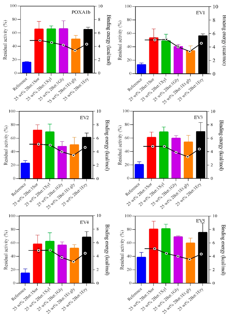
Figure 3. Comparison of thermostability of 1.25 g L -1 laccases in 50 mM phosphate buffer, pH 7 aqueous solution in the absence and in the presence of 25 wt % betaine-based NADES obtained using five different HBDs after 60 min at 70 °C (histograms), and the binding energy (kcal mol -1 ) between laccases and polyol molecule of NADES calculated using the YASARA structure (dots). The residual activity (%) is determined by comparing the activity measured after 60 min with the free-NADES phosphate buffer, pH 7.0 and 50 mM at 25 °C (reference, 100%).
