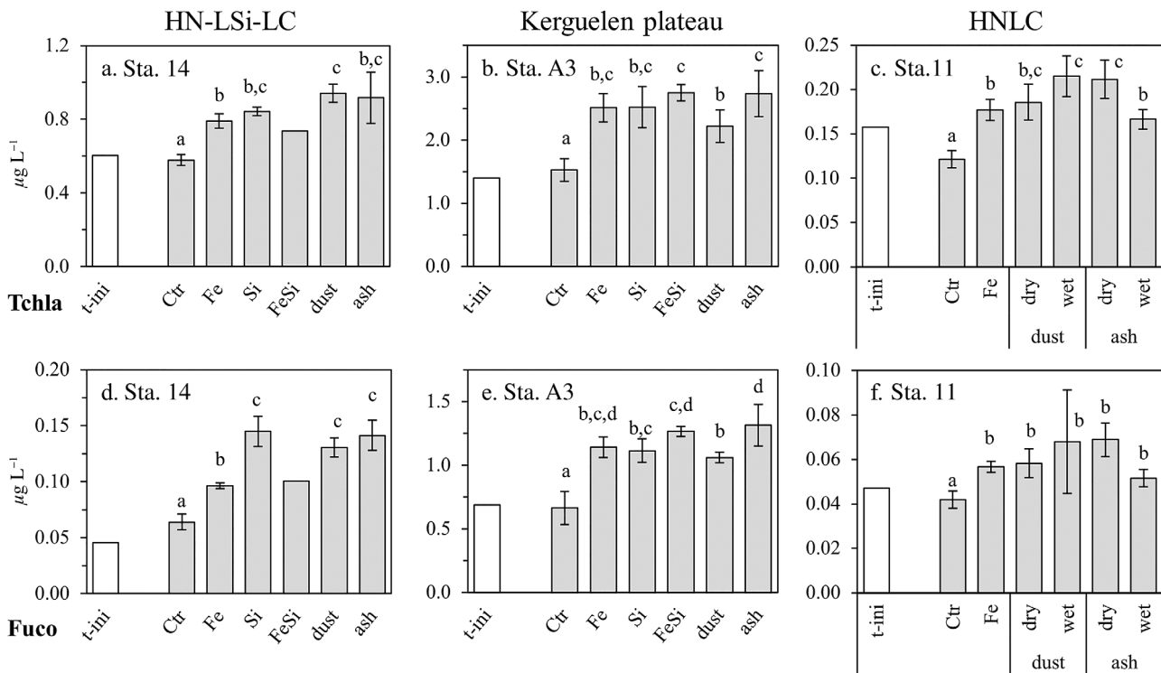
Fig. 4. Pigment concentration ( \mu\text{g L}^{-1} ) of total chlorophyll a ( a–c ) and fucoxanthin ( d–f ) at the beginning of the experiment (t-ini, white bars) and after 48 h of incubation for each treatment at HN-LSi-LC Sta. 14 ( a,d ), plateau Sta. A3 ( b,e ) and HNLC Sta. 11 ( c,f ). Error bars indicate standard deviation of triplicates. FeSi treatment at Sta. 14 is not included in statistics, due to n = 1 . Means that are not significantly different ( p > 0.05 ) are labeled with the same letter within a station.
