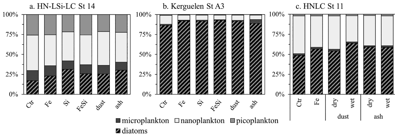
Fig. 5. Size depending relative contribution to Tchl a increase (%) after 48 h of incubation for each treatment relative to control at HN-LSi-LC Sta. 14 ( a ), Kerguelen Sta. A3 ( b ) and HNLC Sta. 11 ( c ), with microplankton (dark), nanoplankton (light), and picoplankton (medium gray). Diatom contribution within the microplankton size fraction is dashed.
