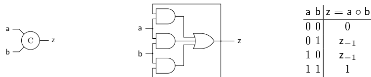
Fig. 1. A Muller c-element symbol (left), a gate-level design (middle) and its truth table (right).
