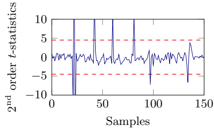
Fig. 14. 2 nd order TVLA results for the 1 st order masked AES S-box based on one million simulated traces.
