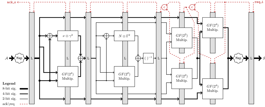
Fig. 10. Self-timed AES S-box based on the Canright's design.
