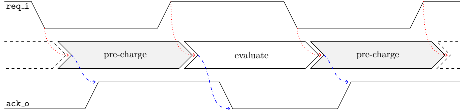
Fig. 4. Self-timed handshake in a pre-charge / evaluate logic.
