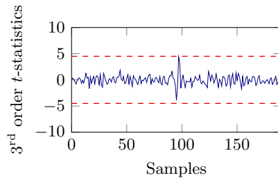
Fig. 16. 3 rd order TVLA results for the 2 nd order masked AES S-box based on one million simulated traces.
