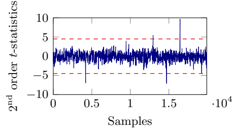
Fig. 18. 2 nd order TVLA results for the 1 st order masked AES encryption based on one hundred thousand simulated traces.
