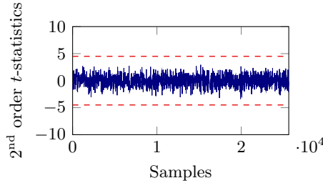
Fig. 19. 2 nd order TVLA results for the 2 nd order masked AES encryption based on one million simulated traces.
