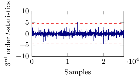
Fig. 20. 3 rd order TVLA results for the 2 nd order masked AES encryption based on one million simulated traces.
