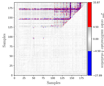
Fig. 21. Bivariate analysis of the 2 nd order self-timed AES S-box implementation. The lower triangle shows the 2 nd order t -test using one million traces with mask refresh enabled. The upper triangle shows the 2 nd order t -test using one hundred thousand traces with mask refresh disabled.
