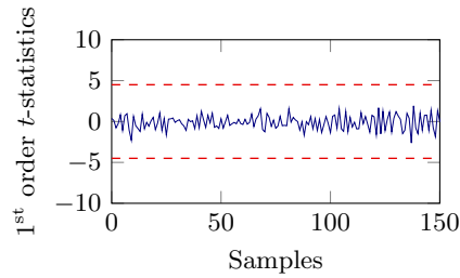
Fig. 13. 1 st order TVLA results for the 1 st order masked AES S-box based on one million simulated traces.
