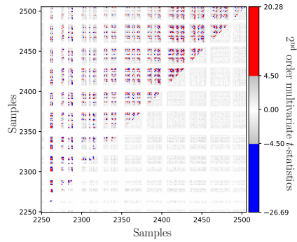
Fig. 22. Bivariate analysis of the 2 nd order self-timed AES encryption implementation. The lower triangle shows the 2 nd order t -test using one hundred thousand traces with mask refresh enabled. The upper triangle shows the 2 nd order t -test using ten thousand traces with mask refresh disabled.
