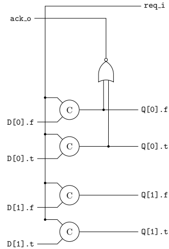
Fig. 3. A 2-bit wide weakly indicating asynchronous latch.
