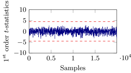
Fig. 17. 1 st order TVLA results for the 1 st order masked AES encryption based on one hundred thousand simulated traces.
