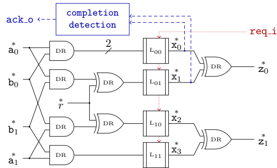
Fig. 9. The 1 st order self-timed DOM gadget.
