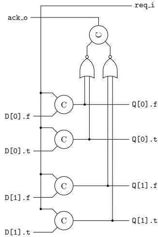
Fig. 2. A 2-bit wide strongly indicating asynchronous latch.
