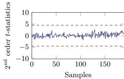
Fig. 15. 2 nd order TVLA results for the 2 nd order masked AES S-box based on one million simulated traces.
