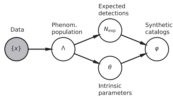
Figure 1. Bayesian graph for comparing synthetic binaries with phenomenological reconstructions of populations from real data. Each node represent a random variable, the shaded node indicates observed data. Each connection between a node and its parents indicates a conditional probability of that node given its parents.
