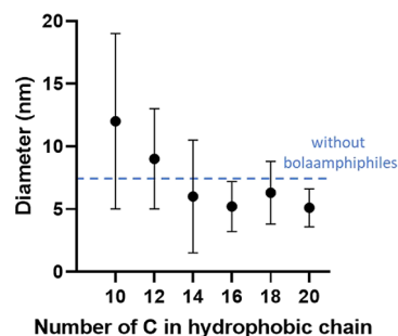
Figure 5. Evolution of the average diameter of AuNPs formed in situ by addition of a \text{NaBH}_4 solution upon a mixture of bolaamphiphiles and \text{HAuCl}_4 ( [\text{Au}]_{\text{final}} = [\text{BolaAla-}C_n] = 5 \times 10^{-4} \text{ mol}\cdot\text{L}^{-1} ).
