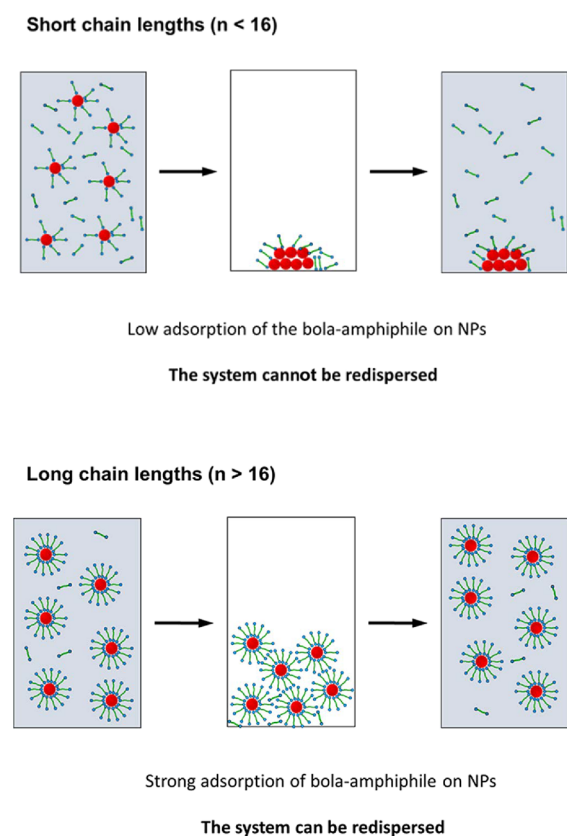
Figure 4. Proposed mechanism of redispersion depending on the alkyl chain length.
