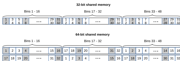
Fig. 15 The figure illustrates how the shared memory banks are accessed if advanced caching mode is used, see Sect. 6.4. The presented layout is employed to reconstruct area of 32 × 32 pixels. The grayed boxes indicate the banks accessed by a warp during the first caching pass. Two values are cached for each bin and, consequently, each bin spans over two memory banks on the platforms with 32-bit shared memory. On these platform it is also only necessary to avoid conflicts within a half-warp. So, the accesses for second half-warp are not shown
