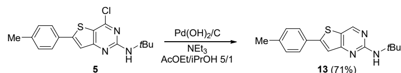
Scheme 5. Synthesis of 4-unsubstituted thienopyrimidine 13 .
