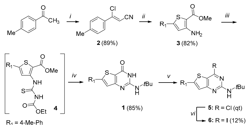
Scheme 1. Synthesis of 4-halogenothienopyrimidines 5 and 6 . Reagents and conditions: (i) 1. \text{POCl}_3 , DMF, RT; 2. \text{NH}_2\text{OH}\cdot\text{HCl} , RT, and 1 h 30; (ii) \text{MeONa} , \text{HSCH}_2\text{CO}_2\text{Me} , \text{MeOH} , 80^\circ\text{C} , and 40 min; (iii) \text{SCNCO}_2\text{Et} , DMF, 30^\circ\text{C} , and 2 h; (iv) 1. t\text{BuNH}_2 , \text{Net}_3 , \text{EDCl}\cdot\text{HCl} , DMF, RT, and 18 h; 2. 170^\circ\text{C} and 2 h; (v) \text{POCl}_3 , N,N -dimethylaniline, \text{ACN} , 85^\circ\text{C} , 16 h; 2. \text{H}_2\text{O} , 40^\circ\text{C} , and 2 h; (vi) \text{NaI} , dioxane, and reflux.
