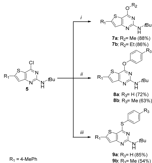
Scheme 2. Synthesis of O -alkyl, O -aryl, and S -aryl derivatives 7–9 . Reagents and conditions: (i) \text{R}_2\text{ONa} , \text{R}_2\text{OH} , 60^\circ\text{C} , 6–22 h; (ii) \text{R}_3\text{-PhOH} , \text{K}_2\text{CO}_3 , DMF, 130^\circ\text{C} , 3 h; (iii) \text{R}_3\text{-PhSH} , \text{K}_2\text{CO}_3 , DMF, 1 h 30, 30^\circ\text{C} .
