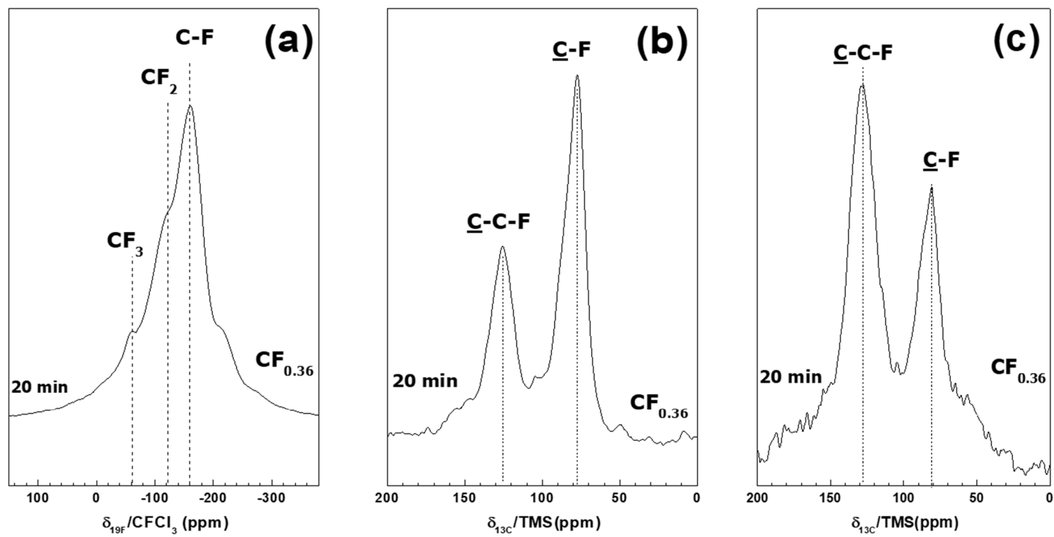
Figure 5: Spectra of fluorinated MOF, (a) ^{19}\text{F} Magic Angle Spinning [MAS] 14 kHz NMR spectrum, (b) ^{19}\text{F} \rightarrow ^{13}\text{C} Cross Polarization [CP] NMR spectrum and ^{13}\text{C} MAS 10 kHz NMR spectrum (c).
