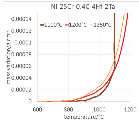
Figure 2: Start of oxidation during heating as detected by mass gain after correction from air buoyancy variation
