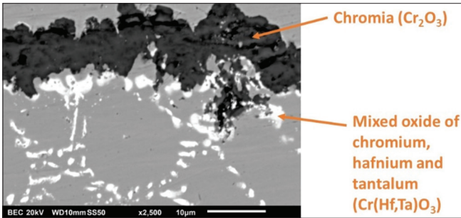
Figure 11: Identification of the formed oxides by high magnification scanning electron microscope/backscattered electrons mode imaging (here the alloy oxidized at 1100°C and observed at ×2500)
