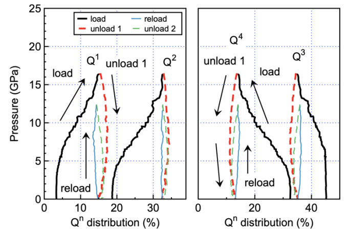
Fig. 5: silica speciation in MD simulation for 0.3\text{Na}_2\text{O}-0.7\text{SiO}_2 glass as a function of pressure, during two successive pressure cycles with P_{max} = 16.4 GPa and 12.4 GPa.
