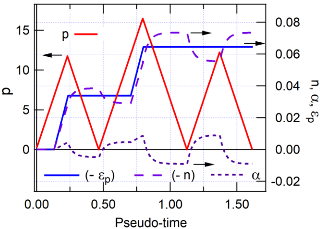
Fig. 4: History of pressure p as a function of pseudo-time (defined from elastic strain), densification -\varepsilon_p , internal variable \alpha and the spectroscopic variable -n = -\varepsilon_p - \alpha
