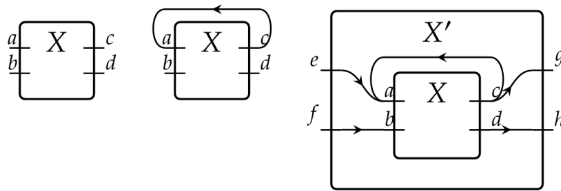
Figure 4: From left to right: a box X , an invalid-box X and an arrow X \rightarrow X'
