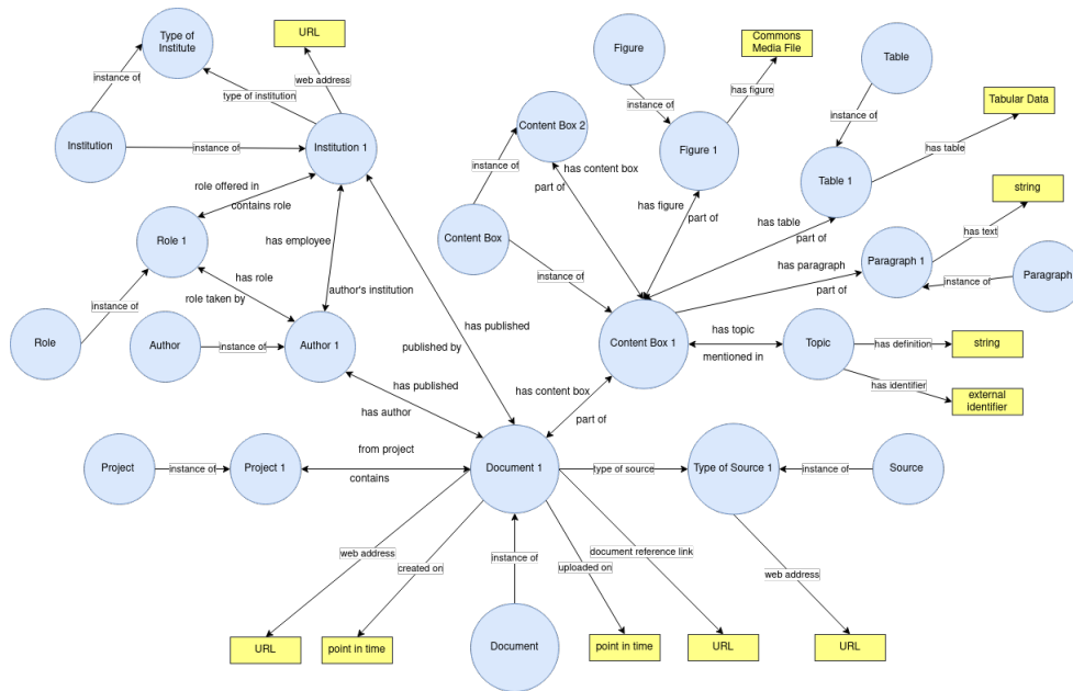
Figure 1: Ontology to represent the documents in Wikibase
