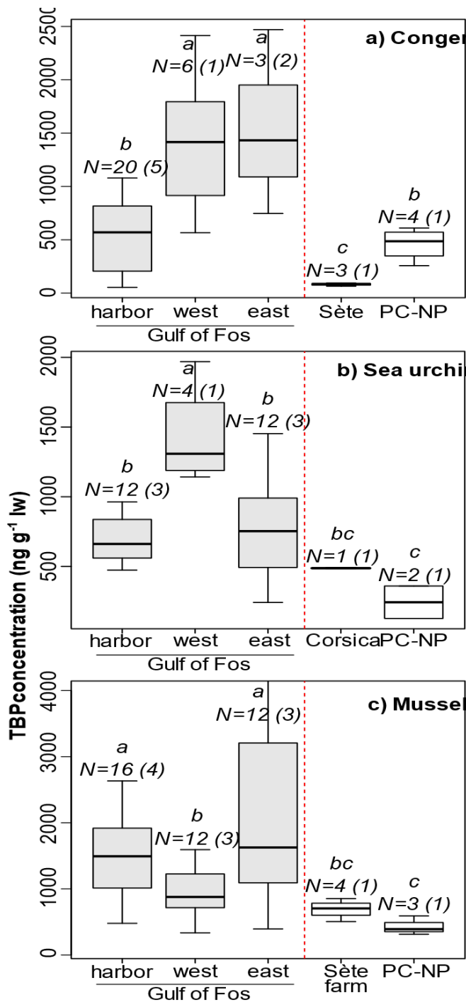
Figure 4. TBP concentration levels (medians, quartiles and 1.5*interquartile ranges) in the defined zones of the Gulf of Fos (grey), and more remote locations along the French Mediterranean (white) for A) European conger, B) sea urchin, and C) mussel.
