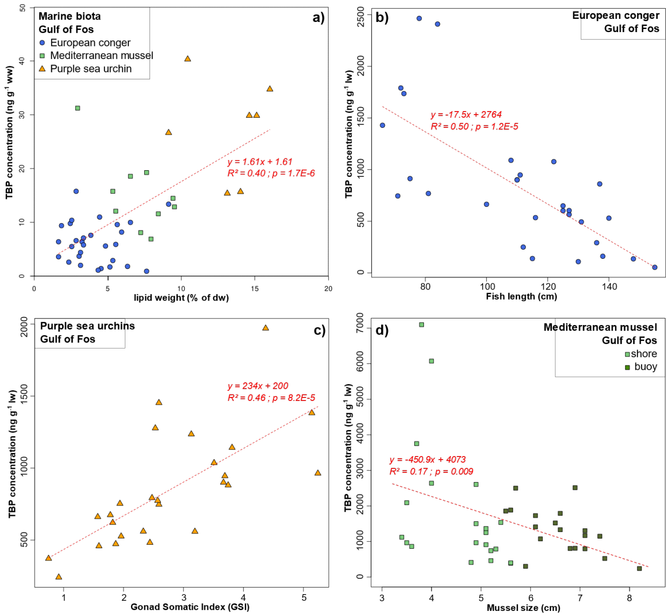
Figure 3. Correlations between a) all species TBP levels ( \text{ng g}^{-1} \text{ ww} ) and lipid weight (% of dw), b) European conger TBP levels ( \text{ng g}^{-1} \text{ lw} ) and fish length (cm), c) purple sea urchins TBP levels ( \text{ng g}^{-1} \text{ lw} ) and gonad somatic index (GSI), and d) Mediterranean mussel TBP levels ( \text{ng g}^{-1} \text{ lw} ) and shell size (cm). Urchin and mussel concentrations in a) are pooled, in c) and d) include all sub-samples concentrations.
