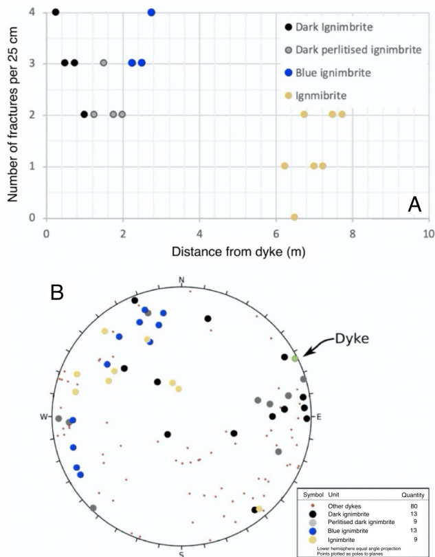
Figure 3: [A] Fracture spacing data recorded at scan-line intersection binned every 25 cm to illustrate fracture density as a function of distance from the dyke margin. [B] Stereographic lower hemisphere, equal area projection of fracture orientations planes in the different rock types including comparison to the orientation of the dyke investigated in this study and other dykes in Hvítserkur measured in the field.
