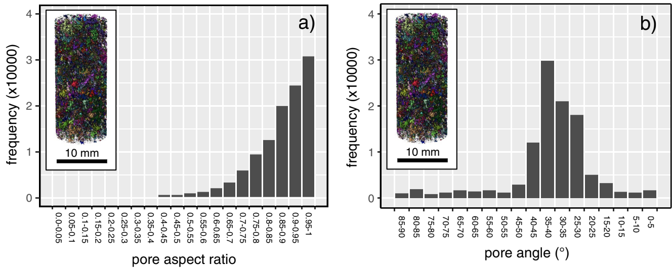
Figure 9. Histograms of (a) pore aspect ratio (the ratio of the minor to the major pore axis, where a value of unity represents a sphere) and (b) pore angle (the angle of pore major axis, where 90° is parallel to the axis of the cylindrical sample) for intact Volvic trachyandesite. This pore shape analysis was performed on the pores not connected to the porosity backbone (i.e., the image volume shown in Figure 2d). The insets show an image of the segmented 3D X-ray CT volume used for the analysis.
