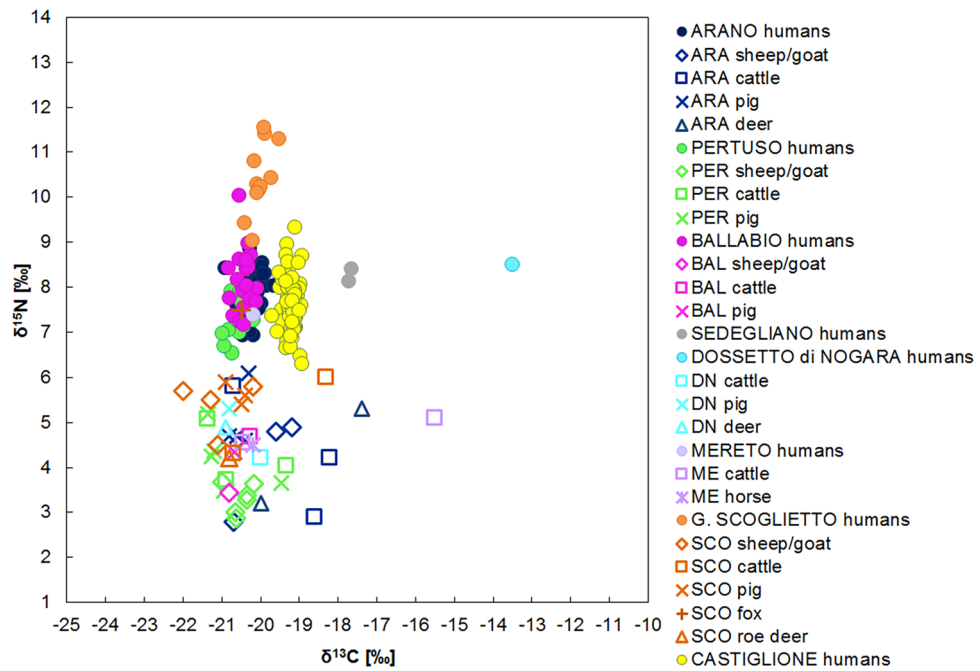
Figure 2. The \delta^{15}\text{N} and \delta^{13}\text{C} human and animal values for the Italian Early Bronze Age sites.
