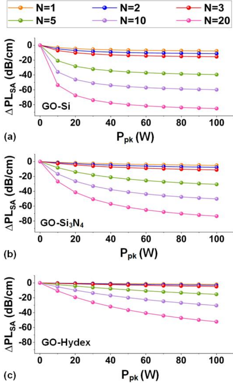
Figure 5. Excess propagation loss induced by the SA ( \Delta PL_{SA} ) versus peak power of input optical pulses ( P_{pk} ) for (a) Si, (b) Si 3 N 4 , and (c) Hydex waveguides coated with different numbers of GO layers.
