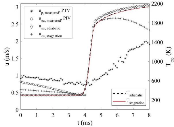
FIG. 6: Temporal evolution of the droplet velocity (PTV) and the measured (PIV) and computed gas velocities in stoichiometric condition ( d_0=47\ \mu\text{m} )
