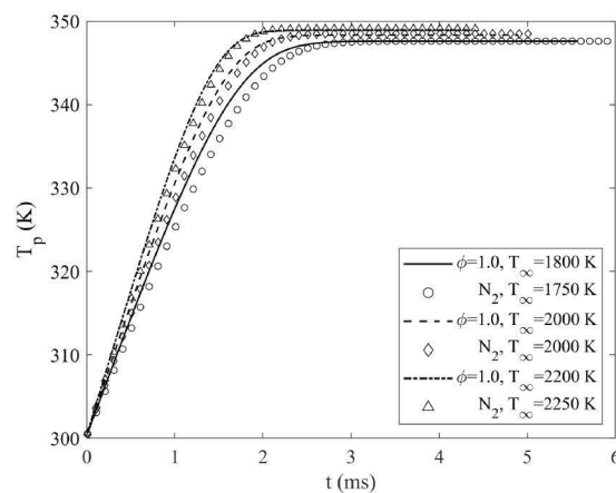
FIG. 8: Temporal evolution of the droplet temperatures at high temperature conditions
