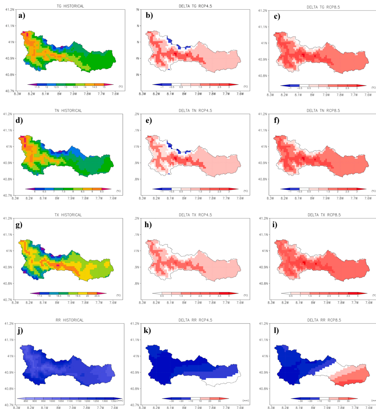
Fig. 3. Spatial distribution of climate variables in the Paiva catchment: a) annual mean temperature; b) mean temperature change under RCP4.5; c) mean temperature change under RCP8.5; d) annual minimum temperature; e) minimum temperature change under RCP4.5; f) minimum temperature change under RCP8.5; g) annual maximum temperature; h) maximum temperature change under RCP4.5; i) maximum temperature change under RCP8.5; j) mean annual precipitation; k) mean precipitation change under RCP4.5 and l) mean precipitation change under RCP8.5.
