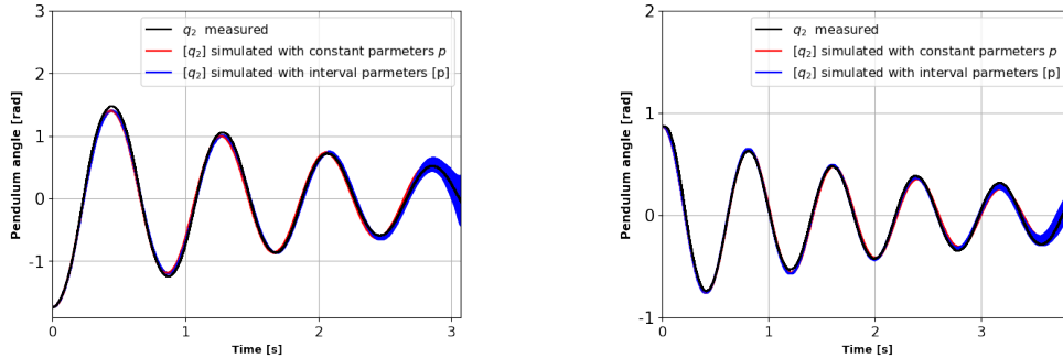
(a) Initial conditions: [\mathbf{u}_0] = [0 \text{ Nm}, 0 \text{ Nm}] and [\mathbf{x}_0] = [0^\circ, 0^\circ] \times [0, 0] \times [-98^\circ, -100^\circ] \times [0, 0] . [x_{10}] \quad [x_{20}] \quad [x_{30}] \quad [x_{40}] (b) Initial conditions: [\mathbf{u}_0] = [0.15 \text{ Nm}, 0.18 \text{ Nm}] and [\mathbf{x}_0] = [0^\circ, 0^\circ] \times [0, 0] \times [46^\circ, 50^\circ] \times [0, 0] . [x_{10}] \quad [x_{20}] \quad [x_{30}] \quad [x_{40}]
