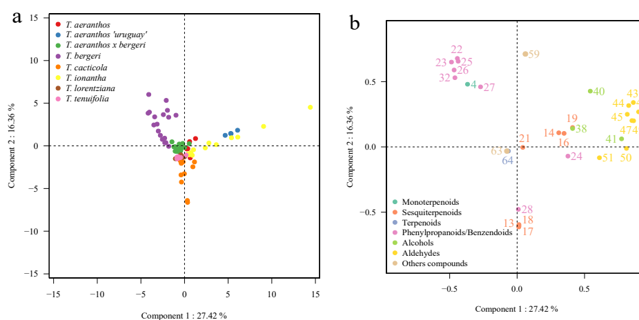
Figure 3. PCA based on VOCs emitted by T. aeranthis , T. bergeri , T. aeranthis x T. bergeri (the hybridization of the two species), T. aeranthis 'uruguay', T. cacticola , T. ionantha , T. lorentziana , and T. tenuifolia . (a) Score plot of PC1 scores versus PC2 scores. (b) Loading plot of PC1 and PC2 contributing volatile compounds. Numbers in (b) correspond to the compounds numbers listed in Table 2.
