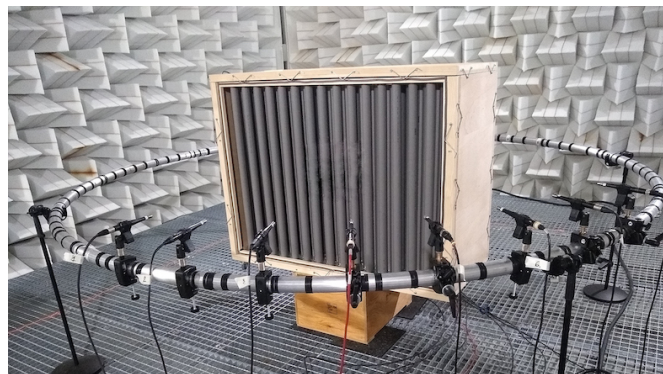
(a) Proxy buffet in anechoic chamber.
