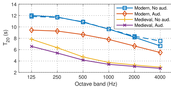
Figure 2 – Estimated T_{20} as a function of frequency band, averaged across sixteen positions evenly distributed along the Great Chapel. For the modern, unoccupied state, the measured (---) and modeled (—) T_{20} s are shown.
