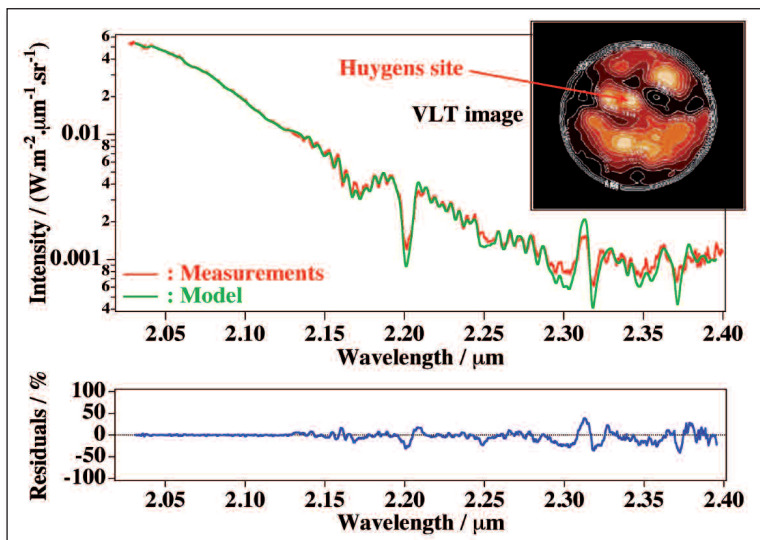
▼ FIG. 5: Upper right: VLT (Very Large Telescope) image. Bright zones correspond to high albedo regions. Top: Measured spectrum around the Huygens landing site with a resolving power of 700 (in red) and simulated spectrum (in green). Bottom: relative difference between measurements and the best model (in blue). Above 2.12 \mu\text{m} , the measurement error is \pm 27\% . The vertical haze profile and the surface albedo at 2 \mu\text{m} were determined from these measurements.
