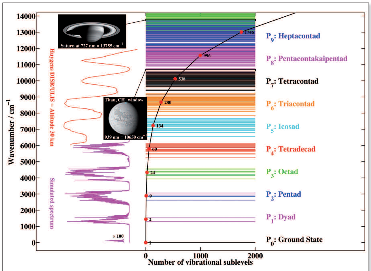
► FIG. 2: Methane's spectrum complexity. Horizontal lines represent vibration energy levels. The black curve gives the number of vibrational sublevels for each polyad. The names correspond to the different absorption bands. Different spectral regions are illustrated by images and spectra: in pink, a simulated spectrum for lower polyads and, in red, an example of the spectra recorded on Titan by the Huygens probe. © NASA/JPL/Space Science Institute).
