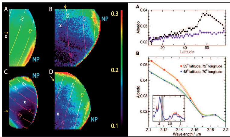
▲ FIG. 4: Left: Albedo (proportion of reflected solar light) maps of Titan at 2.8 \mu\text{m} obtained by the VIMS instrument of the Cassini spacecraft. Red areas have highest albedo. The red spot near the North Pole (NP) is an ethane cloud. Upper right: Albedo as a function of latitude at 2.11 \mu\text{m} (in black) and 2.17 \mu\text{m} (in magenta), revealing the diffusion by the cloud that is visible at 2.11 \mu\text{m} beyond 51°N. Lower right: measured (dots) and simulated (curves) spectra at two different latitudes. The difference between spectra at these two latitudes reflects the diffusion by the ethane cloud that is situated around 30 to 50 km altitude. Figure from Reference [2].
