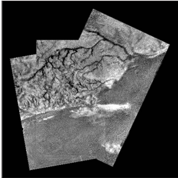
► FIG. 1: "Dried" methane rivers imaged by the Huygens probe during its descent on Titan. © NASA/JPL/Space Science Institute.
