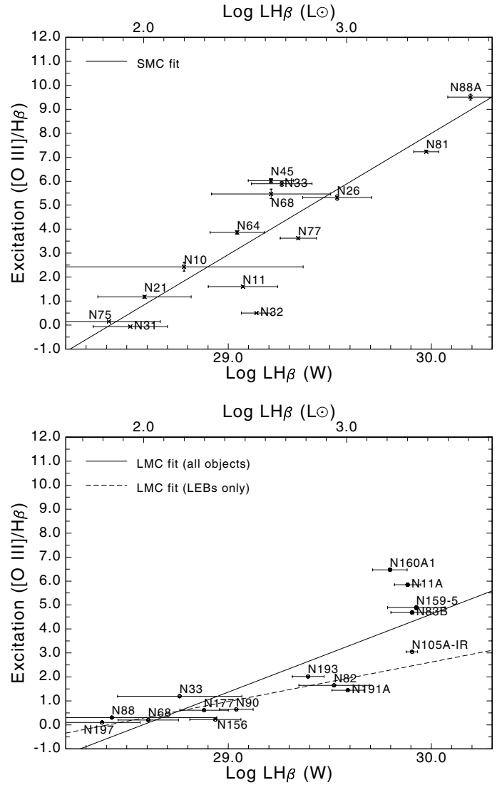
Fig. 2. Excitation (measured by the line ratio [O III] \lambda\lambda 4959 + 5007/H\beta ) versus the H\beta luminosity for the SMC and LMC objects. The logarithmic luminosity scale is in units of watts W, 10^7 \text{ erg s}^{-1} as well as in units of solar bolometric luminosity. The figures are based on the data presented in Tables 3 and 2, respectively. Solid lines: least-square fits for the SMC and LMC objects. Dashed line: least-square fit for the LMC sample, excluding HEBs (filled dots).
