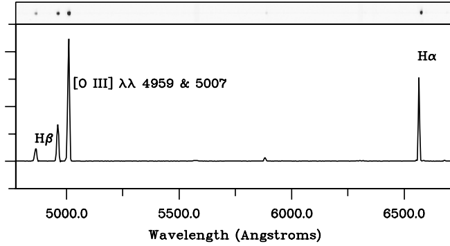
Fig. 1. A sample spectrogram belonging to SMC N88A. The upper panel shows the 2D spectrum and the lower panel a cut through the central row, with relative intensity scale.
