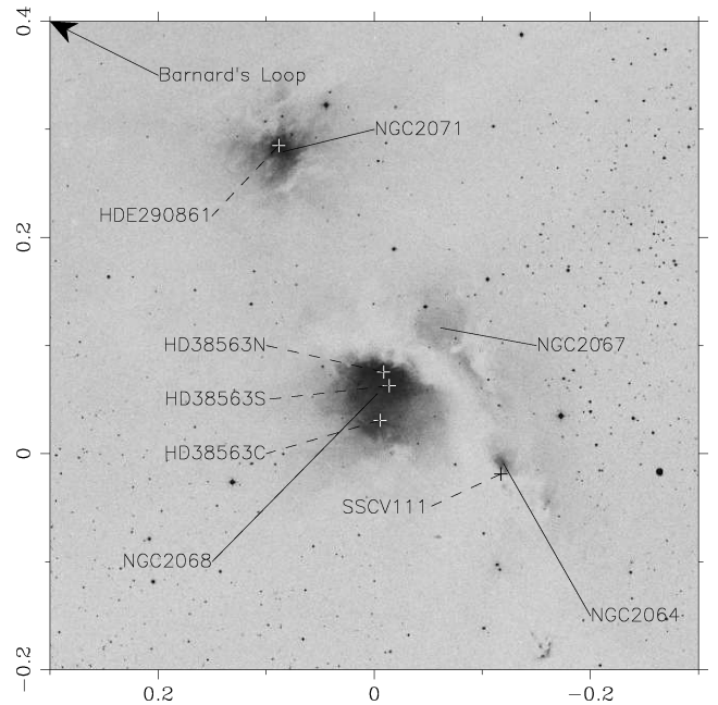
Figure 1. M78 area taken from Digitized Sky Survey (DSS) blue band survey. The largest and brightest nebula is NGC 2068/M78, the arc-shaped nebula to the west is NGC 2067. North-east from NGC 2068 is NGC 2071 and the faintest nebula, south-west from NGC 2068 is NGC 2064. The crosses indicate the positions of the brightest stars in the field. The dashed lines point to these stars and the nebulae are pointed to with solid lines. The coordinates are in right ascension and declination offsets from ( 05^{\text{h}}46^{\text{m}}46^{\text{s}}.7 + 00^{\circ}00'50'' , J2000), in degrees of arc.
