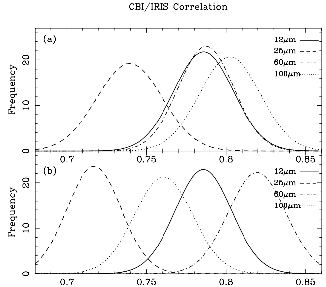
Figure 8. (a) Fitted distributions to Monte Carlo noise simulation of the correlation coefficient r_{\text{sky}} between CBI and IRIS for M78. The solid lines correspond to the 12- \mu\text{m} templates, the dashed lines to 25 \mu\text{m} , the dot-dashed lines to 60 \mu\text{m} and the dotted lines to 100 \mu\text{m} . The Gaussian parameters are listed in Table 2. (b) Distributions obtained from UV-field corrected templates. The corresponding parameters are also listed in Table 2.
