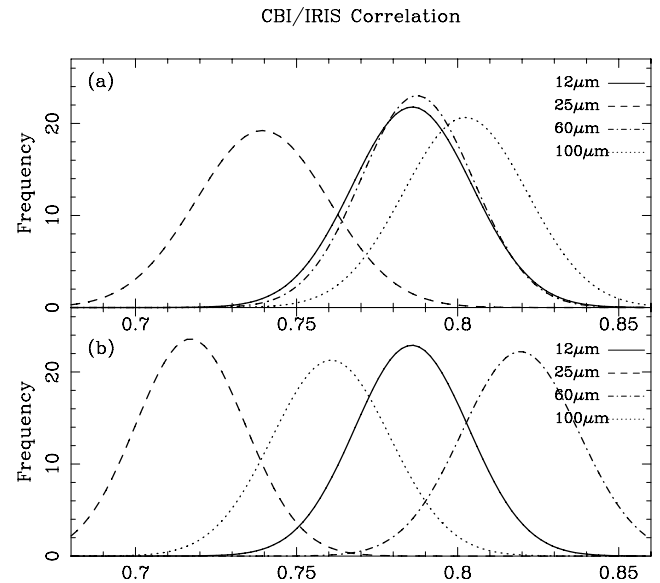
Figure 8. (a) Fitted distributions to Monte Carlo noise simulation of the correlation coefficient r_{\text{sky}} between CBI and IRIS for M78. The solid lines corresponds to the 12- \mu\text{m} templates, the dashed lines to 25 \mu\text{m} , the dot-dashed lines to 60 \mu\text{m} and the dotted lines to 100 \mu\text{m} . The Gaussian parameters are listed in Table 2. (b) Distributions obtained from UV-field corrected templates. The corresponding parameters are also listed in Table 2.
